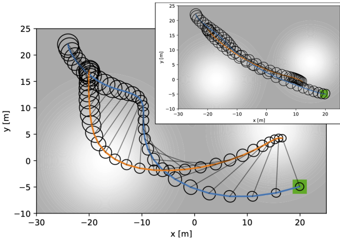
Fig. 4. Guide dog (orange) with leash (black line) guides the blind agent (blue) towards the goal location (green). While doing so it passes by both light sources to reduce the uncertainty of the blind person’s position at the goal location. The top right inset shows the case where the guide dog is indifferent about the blind person’s uncertainty.
