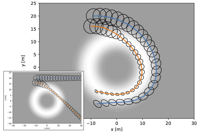
Fig. 2. Agent 1 (blue) is pushing Agent 2 (orange) into the light to reduce the uncertainty over Agent 2 at the end of the planning horizon. Uncertainties are visualized by covariance ellipses. Both agents are initialized with positive velocity in the x-direction.
