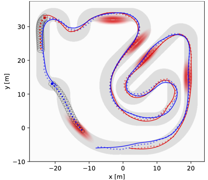
Fig. 1. One application we present is dynamic racing. Here, the blue agent starts with a disadvantage but is equipped with better acceleration and capable of moving faster through corners than the red agent. Our approach allows the blue agent to overtake and win the race. Planned trajectories and chance constraints are shown in dashed lines and ellipses. The traces correspond to the true state (solid) and the noisy EKF-estimate (dashed) available to each agent during the race. The red areas are zones with low noise observations and reduce uncertainty.
