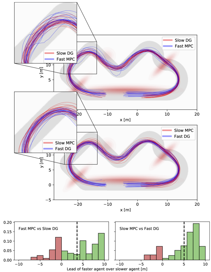
Fig. 7. Top: Traces of agents comparing MPC and DG. In both cases the MPC method moves away from the ideal racing line more often due to failed overtaking attempts. It can not foresee it’s influence on the DG agent’s actions and thus is less efficient. It is also not able to take advantage of estimating is implicit control over the other agent like the DG agent. The agents start from random initialization locations around the origin. Bottom: Histograms of the \Delta arc-length lead of the faster agent over the slower agent. Green indicates that the faster agent won the race against the agent starting in the lead, whereas red indicates the opposite. In comparison, the DG method won more races than the MPC method and had a higher average lead.
