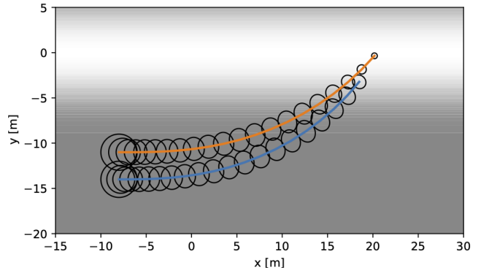
Fig. 2. Agent 1 (blue) is pushing Agent 2 (orange) into the light to reduce the uncertainty over Agent 2 at the end of the planning horizon. Uncertainties are visualized by covariance ellipses. Both agents are initialized with positive velocity in the x-direction.
