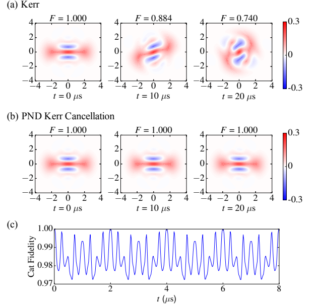
FIG. 5. Simulated evolution of the cavity cat state \frac{1}{\sqrt{2}}(|\alpha_c\rangle + |-\alpha_c\rangle) , an even superposition of coherent states with opposite phases. (a) Wigner-function snapshots and the fidelity F of the cat state evolving under the cavity self-Kerr. (b) Wigner-function snapshots and the fidelity F of the cat state with PND Kerr cancellation. (c) Cat-state fidelity as a function of time under PND Kerr cancellation, showing a clear signature of the micromotion. Here we use parameters in table VII and assume \alpha_c = \sqrt{2} , cavity photon number N_{\text{cut}} = 6 , \chi/2\pi = 2 MHz, and T_M = 2\mu\text{s} .
