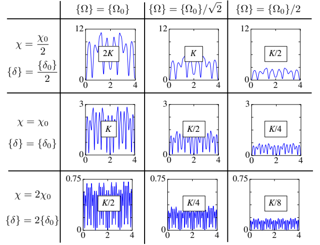
FIG. 10. Micromotion of the cat-state infidelity under PND Kerr cancellation. In this table of plots we show the infidelity (y-axis, %) of a cat state (cat size \alpha_c = \sqrt{2} ) as a function of time (x-axis, \mu s) with varying sets of parameters \chi, \{\Omega\} , and \{\delta\} . The insets indicate the corresponding cavity self-Kerr value with K/2\pi = 3 kHz. Here we assume abrupt PND drive, and \chi_0, \{\Omega_0\} , and \{\delta_0\} are the parameters in Table VII. One can clearly infer that the micromotion amplitude scales as |\Omega^2/\chi^2| and that the micromotion period is T_M = 8\pi/\chi as predicted.
