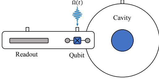
FIG. 1. Schematic of the cQED implementation of a coupled qubit-cavity system, where a transmon qubit is capacitively coupled to a three-dimensional (3D) microwave cavity resonator. One can apply control drives on the transmon qubit through a drive port, and the qubit can be coupled to an additional quasipolar resonator for readout.
