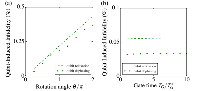
FIG. 4. Qubit-induced infidelity of the PND R_\theta gate. (a) Qubit-induced infidelity as a function of the rotation angle \theta , with fixed PND drive parameters \chi_0, \{\Omega_0\}, \{\delta_0\} and with a \theta -dependent gate time T_G = (40/\pi)T_G^* . (b) Qubit-induced infidelity as a function of the gate time T_G , with fixed parameters \theta = \pi/4, \chi_0, \{\delta_0\} , and with T_G -dependent drive amplitudes \{\Omega\} = \{\Omega_0\sqrt{T_G^*/T_G}\} . Here \chi_0, \{\Omega_0\} , and \{\delta_0\} are the parameters in table V. We assume \Gamma_q/2\pi = \Gamma_\phi/2\pi = 3 kHz, and T_G^* = 16\pi/\chi = 3.125 \mu\text{s} . The initial state is (1/\sqrt{2})(|0\rangle_k + |1\rangle_k) \otimes |g\rangle , and we assume a smooth ramping function \lambda_{\text{gate}}(t) = \sqrt{2}\sin(\pi t/T_G) for the drive.
