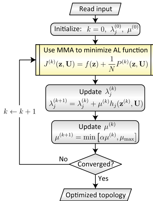
Fig. 3 Schematic flowchart of the AL-based topology optimization framework implemented in this study to solve topology optimization problems with local stress constraints
