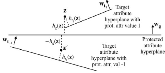
Figure 7: Computing z' when the target attribute hyperplanes for each protected attribute class are very different.
