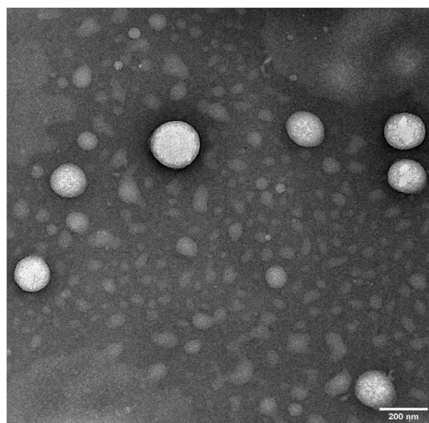
Figure 6. Transmission electron microscopic image of optimized ciprofloxacin nanoemulsion formulation. Image was taken at \times 25 k magnification.
