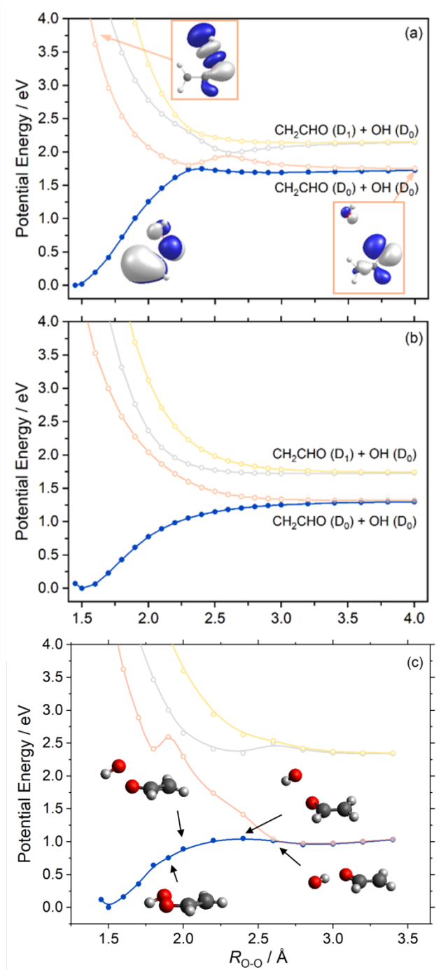
Figure 5: unrelaxed adiabatic PE profile of VHP along the O-O stretch coordinate at (a) \tau_{CCOO} = 0^\circ and (b) \tau_{CCOO} = 90^\circ , calculated at the XMS-CASPT2/aug-cc-pVTZ level of theory. (c) XMS-CASPT2/AVTZ//CASPT2/AVTZ relaxed PE profiles along the R_{O-O} coordinate.
