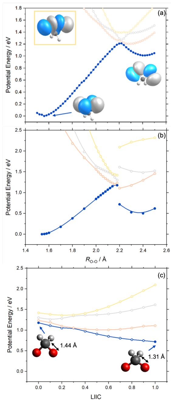
Figure 3: Relaxed PE profiles along the O-O stretch coordinate of dioxirane of the lowest four singlet states, calculated at the (a) MS-CASPT2/AVTZ//MP2/AVTZ and (b) MS-CASPT2/AVTZ//CASPT2/AVTZ levels of theory. The orbitals represent the highest doubly
