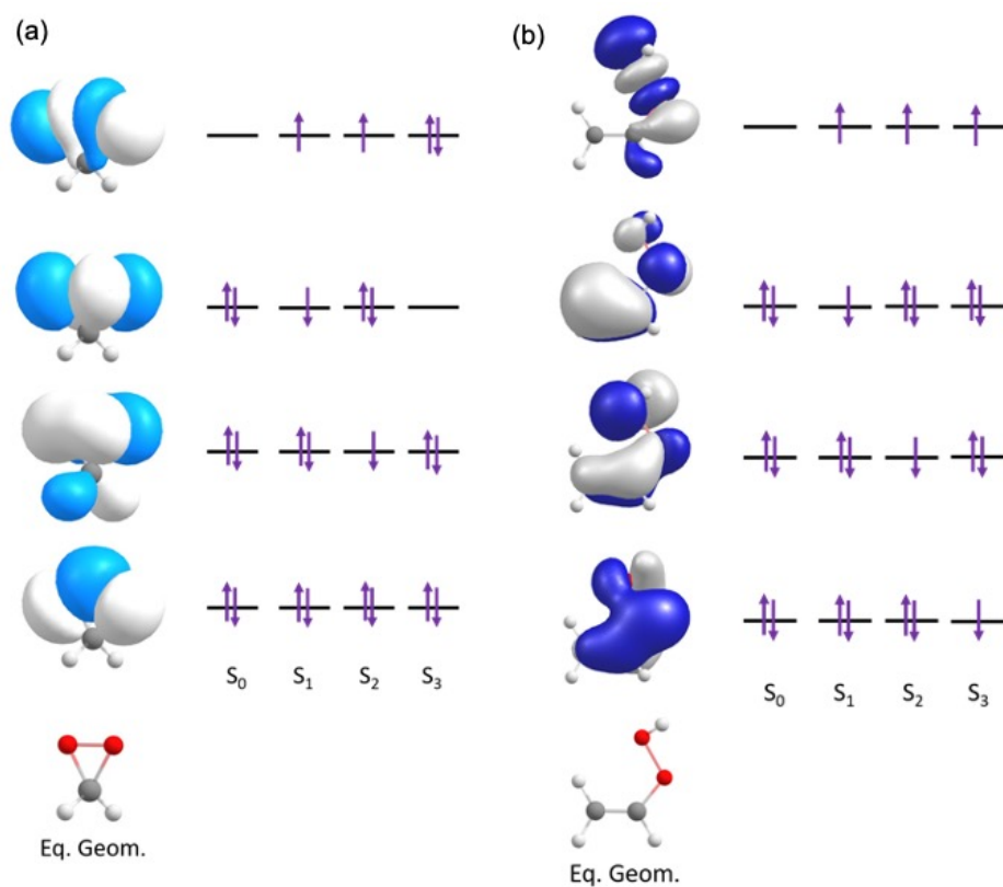
Figure 2: Orbitals and orbital promotions associated with the vertically excited electronic states of (a) dioxirane and (b) VHP.
