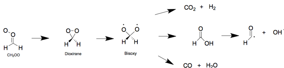
Scheme 1: Reaction mechanism associated with the unimolecular decay of CH 2 OO to form the bisoxy biradical.
