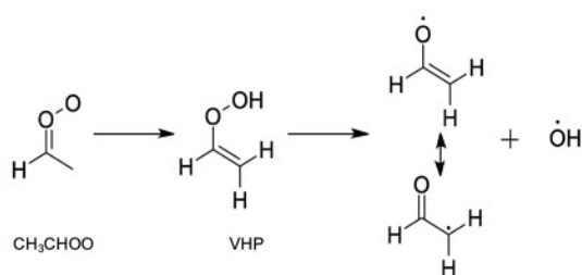
Scheme 2: Reaction mechanism associated with the unimolecular decay of CH 3 CHOO to form the CH 2 CHO + OH radicals via a VHP intermediate.
