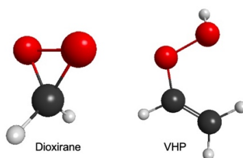
Figure 1: Ground state minimum energy geometry of dioxirane and VHP – calculated at the B2PLYP-D3/6-311+G(d,p) level of theory.
