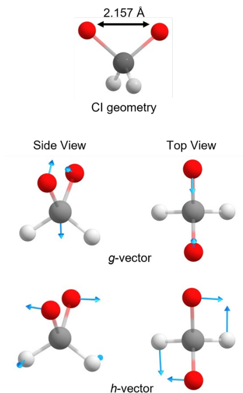
Figure 4: g and h vectors associated with the optimized S_0/S_1 conical intersection of dioxirane
