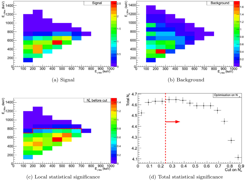
Fig. 11. \gamma -ray 1 energy vs \gamma -ray 2 energy distributions for 2\nu\beta\beta ( 0_{gs}^+ \rightarrow 0_1^+ ) signal simulation (11(a)) and background (11(b)). Local statistical significance distributions for each bin of this histogram (11(c)) with optimisation cut (dotted red line) on total statistical significance N_{\sigma} presented in Fig. 11(d).
