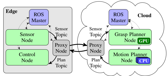
(b) FogROS Application with Proxy
