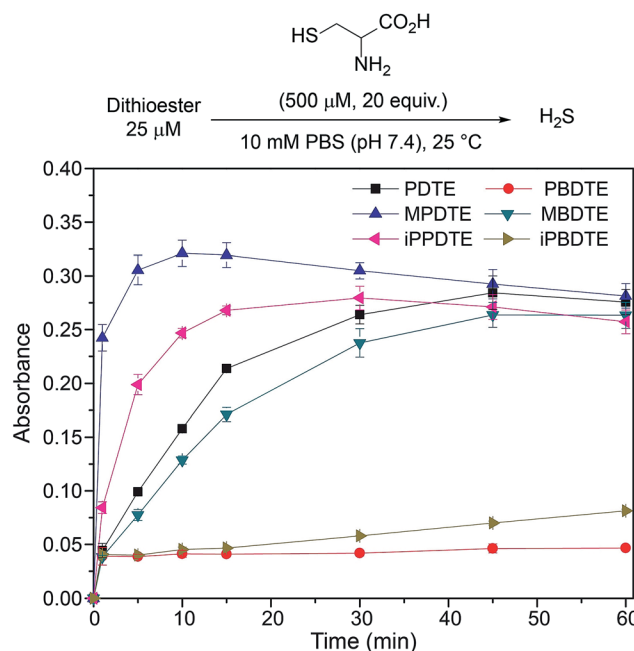
Fig. 7 Effect of alkyl functionalization on the rate of H 2 S release from dithioesters.
