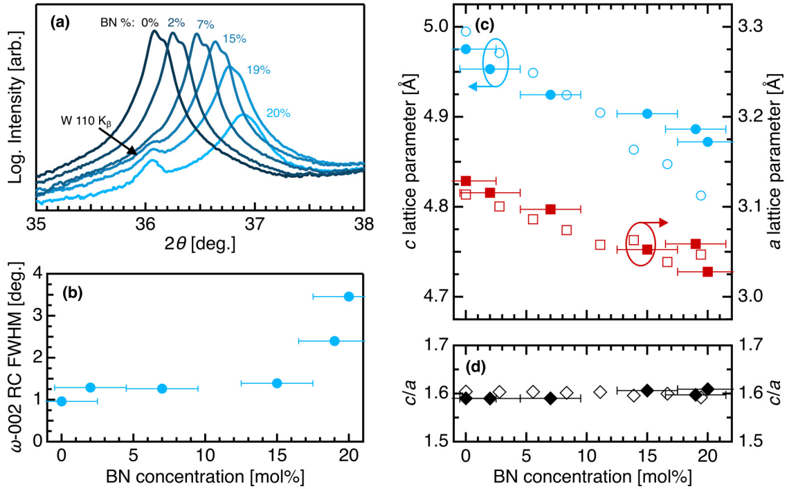
FIG. 4. (a) XRD symmetric \theta - 2\theta scans of the \text{Al}_{1-x}\text{B}_x\text{N} 002 reflection for x = 0.00, 0.02, 0.07, 0.15, 0.19, 0.20 . (b) Rocking curve FWHM values of the \text{Al}_{1-x}\text{B}_x\text{N} 002 reflection for the same films plotted as a function of B concentration. (c) \text{Al}_{1-x}\text{B}_x\text{N} c and a lattice parameters as a function of B concentration, as determined by in- and out-of-plane XRD measurements (filled markers) and first-principles calculations (open markers). The c/a axial ratio is also shown. Error in the measured lattice parameters is smaller than the size of the markers.
