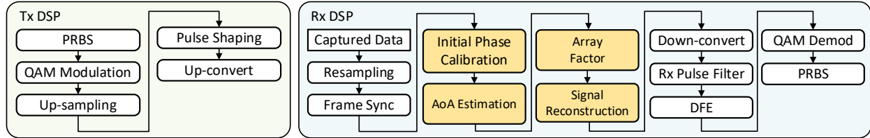
Fig. 2. Workflow of transmitter-side and receiver-side digital signal processing. Digital beamforming steps are shaded in orange color.
