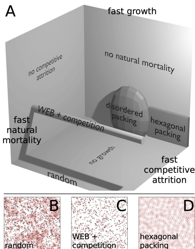
Fig. 3. (A) Schematic 3D realm of models defined on rates of growth, death, and competitive attrition (shadows are generated by a single-point light source at the upper right). WEB theory of allometric forest growth corresponds to fixing population number exponent \alpha = 2 while varying competitive attrition rate (cylinder). Regular hexagonal packing only emerges in a tight limit where growth and death rates approach zero and competitive death rate is high. (B–D) By varying timescales, we obtain spatial patterns qualitatively similar to examples in Fig. 1.
