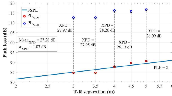
Fig. 10. XPD measurement results using the EVB at 142 GHz and 27 dB. PL_{V-V} measurements follow FSPL and PL_{V-H} for cross-polarized antennas show average XPD of 27.28 dB.
