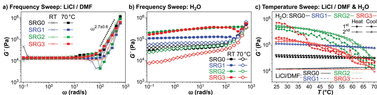
Fig. 2 Rheology of SRG0–SRG3. (a) Frequency sweeps in LiCl/DMF solution at RT and 70^\circ\text{C} . (b) Frequency sweeps in H 2 O at RT and 70^\circ\text{C} . (c) Temperature sweeps in LiCl/DMF and H 2 O at 1 \text{ rad s}^{-1} . All measurements were performed in the linear viscoelastic regime at a strain of 0.05%.
