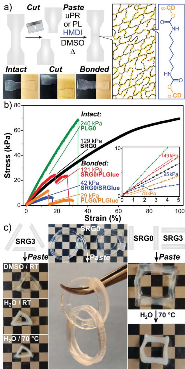
Fig. 4 Cut-and-paste post-gel modifications. (a) Procedure for cutting and re-bonding a dogbone organogel with a heated slide-ring adhesive (SRGlue) solution of uPR/HMDI or a pullulan adhesive (PLGlue) solution of PL/HMDI in DMSO. (b) Tensile tests comparing stress vs. strain in intact and bonded SRG0 and PLG0 dogbone samples with slide-ring adhesive (SRGlue) and pullulan adhesive (PLGlue). The inset magnifies the data in the low-strain region. (c) Photographic examples of SR gels reconfigured by the cut-and-paste approach with SRGlue, showing their stability to thermally triggered volume reduction (left), shape reconfiguration into topological links (center) and hybrid structures derived from different gel formulations (right).
