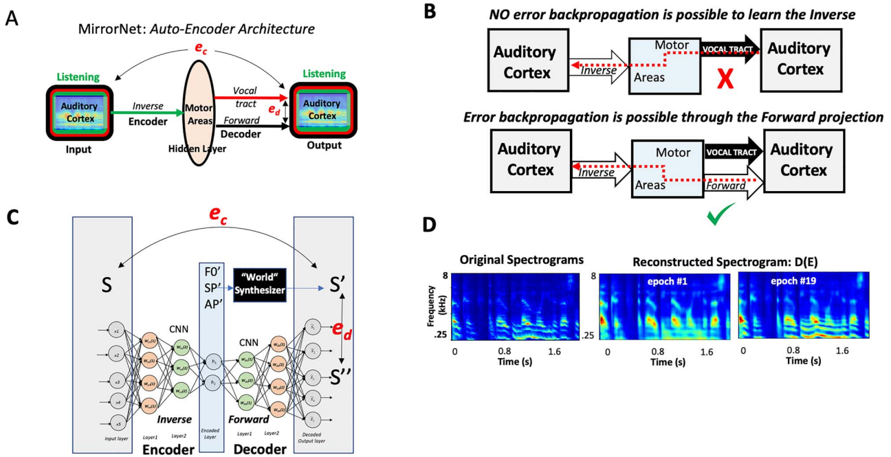
Figure 6. Simulating learning in the Mirror Network. (A) The overall layout of the sensorimotor interactions. It emphasizes the relative contributions of the inverse (Encoder) and forward (Decoder) projections between the auditory and motor areas. The overall network resembles a classic auto-encoder network that maps the auditory cortex activity onto itself through a hidden layer (motor regions), but with an additional non-neural motor-plant (vocal-tract) pathway that shares with the forward projection its motor input and auditory output. Two sources of error are available to train the neural pathways of the Encoder ( e_c ) and Decoder ( e_d ). (B) The critical role of the forward projection in providing a neural pathway for the ( e_c ) error to backpropagate to the motor regions (hidden layers) so as to train the Encoder weights. (C) The MirrorNet implementation employs multiple layers of a convolutional neural network, and the “World” synthesizer as a simplified model of the vocal tract. (D) Training the MirrorNet results in progressive improvements in the reconstructed spectrograms projected through the sequence of Encoder–Decoder layers. The training is rather limited here involving only about 40 min of speech beyond the initialization with the random patterns.
