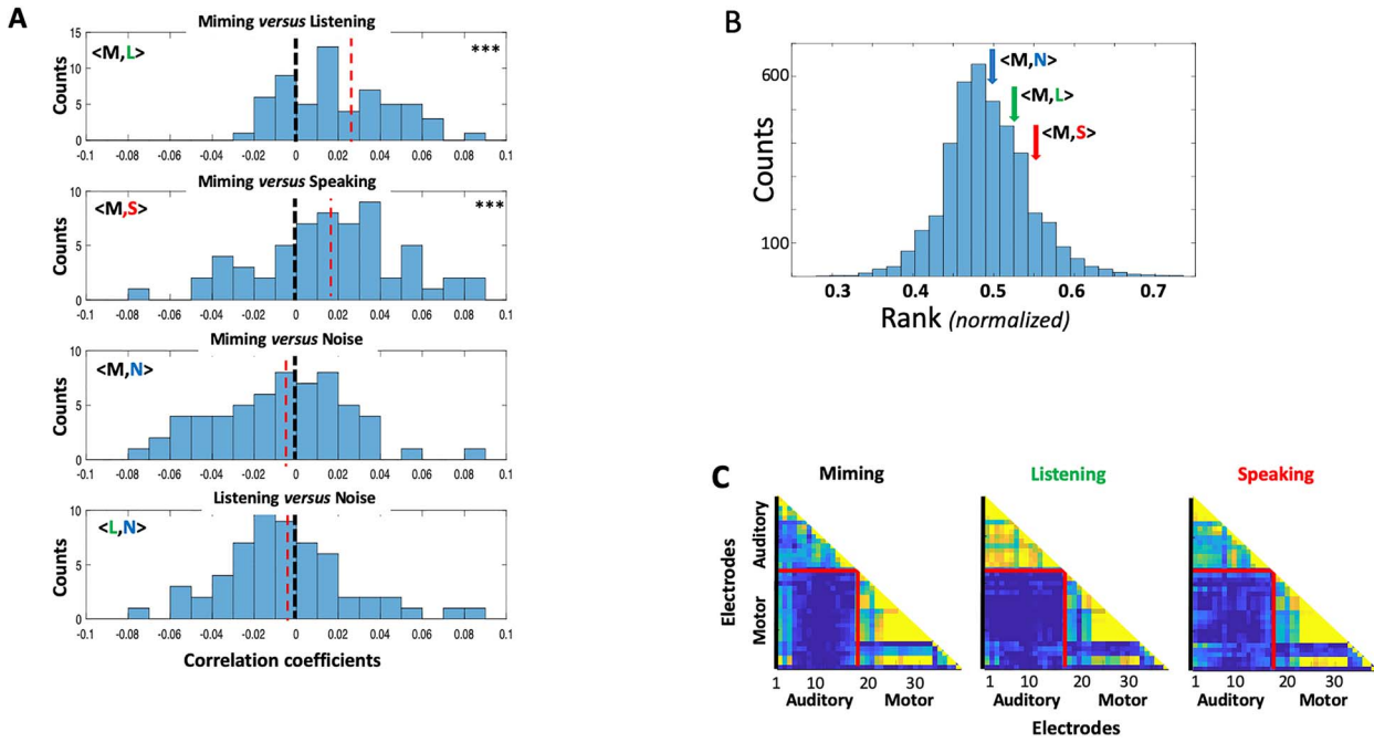
Figure 2. Correlations of auditory-electrode responses in different recording conditions. (A). Distributions of the pairwise correlation-coefficients between M versus L ( \langle M, L \rangle ) and M versus S ( \langle M, S \rangle ) responses to the same speech stimuli, and also M and L versus noise N activity on the same auditory electrodes ( \langle M, N \rangle ) and ( \langle L, N \rangle ). Data are aggregated from all subjects and electrodes. (Top two panels) M responses are positively correlated with L and S responses, and hence the distributions are positively shifted relative to the lower two panels ( P < 0.001 ; 2-sample t-test). (Lower two panels) Neither M nor L are significantly correlated with N . (B) The average rank of correlation coefficients between responses during M and other conditions ( L , S , and N ). The distribution of ranked correlations from randomly ordered responses to different sentences is shown together with the arrows signifying the average \langle M, L \rangle and \langle M, S \rangle on the same sentences. The latter were modestly different from the mean ( 0.63\sigma and 1.13\sigma , respectively) compared with the average of noise response correlations \langle M, N \rangle ( 0.15\sigma ). (C). The correlation coefficients between all pairs of auditory and motor electrodes in subject 3, all measured using the responses within each condition separately. On average, the correlations between the auditory and the motor electrode sets are quite weak compared with within each electrode set. This suggests that the responses across the two electrode regions are of a different nature.
