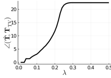
Fig. 2: Plot of the angle (in degrees) between the learned transform and \mathbf{T}_{TV} versus the tuning parameter in (5).
