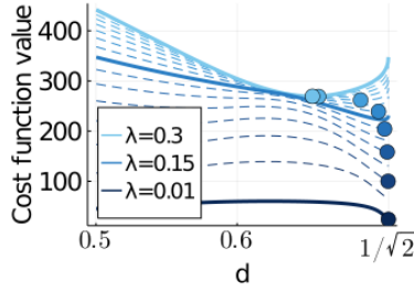
Fig. 1: Plot of the value of the cost function value (5) versus \mathbf{T} as a function of d in (14) for various \lambda s. Smaller values of d mean smoother filters. The points mark \hat{d} .
