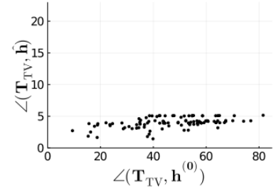
Fig. 3: Scatter plot of the angle between \mathbf{T}_{TV} and the learned filter, \hat{\mathbf{h}} , versus the angle between \mathbf{T}_{TV} and the randomly initialized filter, \mathbf{h}^{(0)} (in degrees).
