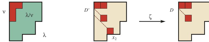
Figure 3.1: Skew Young diagram \lambda/\nu , where \lambda = (5, 5, 5, 4, 4, 2) and \nu = (2, 1, 1) . Map \zeta : D' \rightarrow D , where D' \in \text{ED}(\lambda/\nu) , D \in \text{ED}(\lambda/\mu) , and D' \setminus D = x_2 = (5, 3) .
