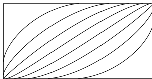
Figure 1.3: The limit curves in a d \times 2d rectangle (created by Dan Romik, April 2020).
