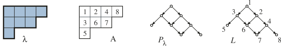
Figure 1.1: Young diagram \lambda = (4, 3, 1) , standard Young tableau A \in \text{SYT}(\lambda) , poset P_\lambda , and the corresponding linear extension L \in \mathcal{L}(P_\lambda) .
