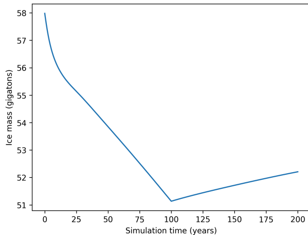
Figure 4. Total ice mass history during retreat (first 100 years) and readvance (second 100 years) of the MISMIP+ experiment.
