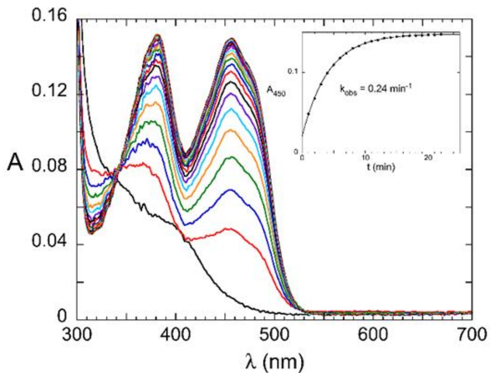
Supplementary Figure 5: Reaction of ThyX with formaldehyde. An anaerobic solution of the thyX•dUMP complex was titrated to complete reduction (2-electrons/FAD) with dithionite. A concentrated solution of formaldehyde was added anaerobically, and UV/visible spectra were scanned every minute in a scanning spectrophotometer. Oxidized enzyme was produced over the course of ~20 minutes at this formaldehyde concentration; its appearance fit a single exponential (inset).
