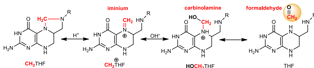
Fig. 1 Hydrolysis reaction of N 5 ,N 10 -methylenetetrahydrofolate as a source of formaldehyde. The cyclic form of CH 2 THF is activated by protonation leading to the iminium species (CH 2 THF + ). This iminium is potentially in equilibrium with its carbinolamine counterpart (HOCH 2 THF). The carbinolamine intermediate can readily decompose into THF and formaldehyde (CH 2 O) in a reversible reaction 28 . CH 2 O can then serve as a direct source of methylene.
