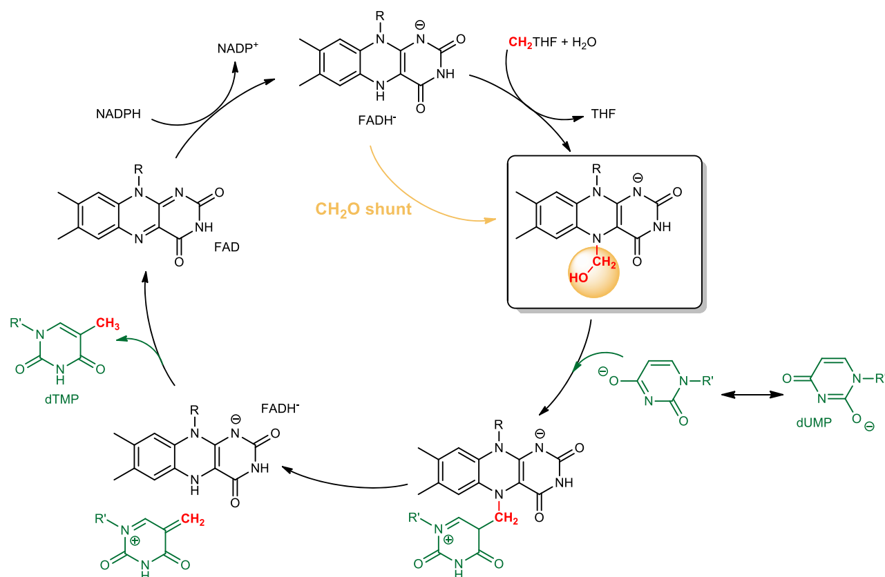
Fig. 4 Proposed chemical mechanism for ThyX. FAD is first reduced by NADPH. Then, the reduced flavin, \text{FADH}^- , reacts with the \text{CH}_2\text{THF} to form a carbinolamine flavin, which acts as the genuine methylene donor. The flavin carbinolamine can be obtained directly via a \text{CH}_2\text{O} -shunt reaction consisting of a reaction of \text{FADH}^- with free \text{CH}_2\text{O} . Methylene transfer from FAD to dUMP is initiated by an \text{S}_\text{N}2 reaction of activated dUMP and the flavin carbinolamine, leading to water elimination and formation of a transient FAD- \text{CH}_2 -dUMP adduct.
