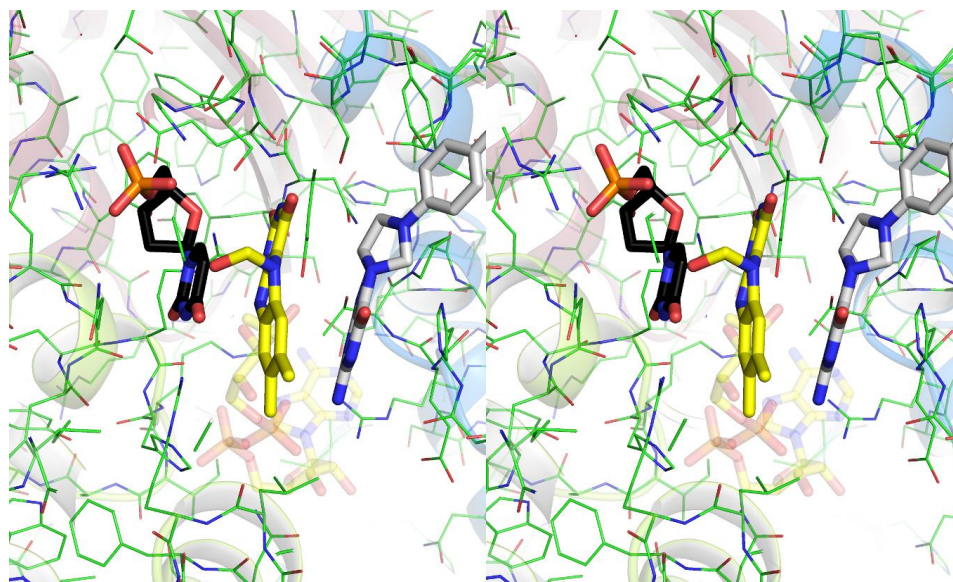
Supplementary Figure 12: Stereo view of a structural model of ThyX in complex with the flavin carbinolamine, dUMP and folate. The model was obtained by superimposing the crystal structure of FADH•CH 2 O complex with the structure of ThyX in complex with dUMP and folate (pdb, 4gt9). The structures used for this model are: (i) ThyX-FADH • soaked with 20 mM CH 2 O vs (ii) pdb 4gt9
