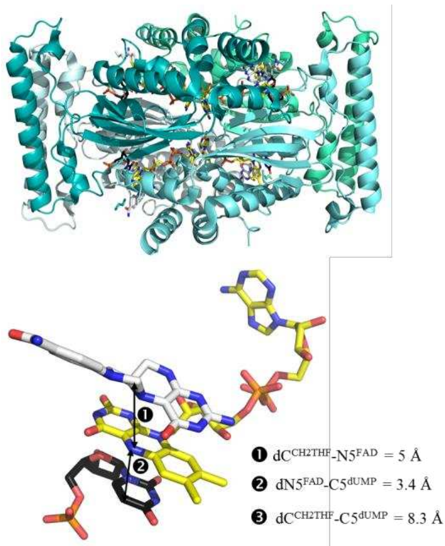
Supplementary Figure 1: Crystal structure of T. maritima ThyX in complex with dUMP and CH 2 THF. Top: 3-D structure representation of homotetramer ThyX (PDB, 4gt9) 1 . The four equivalent active sites, each of them containing an oxidized FAD coenzyme (yellow sticks), a dUMP substrate (black sticks) and a CH 2 THF cofactor (white sticks), are formed at the interface of three monomers. Bottom: Zoom on one of the four active sites showing how FAD, dUMP and CH 2 THF are oriented in ThyX. The atomic distances between the reactive centers are indicated.
