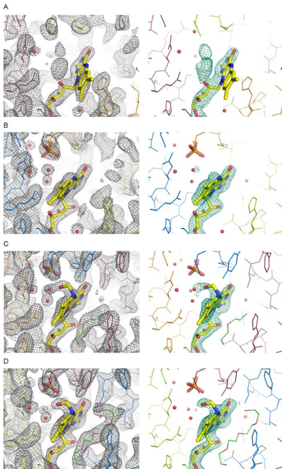
Supplementary Figure 10: Section of the 2mF_o - DF_c electron density (left) and omit map (right) contoured at 1\sigma of the four flavin binding sites observed in the asymmetric unit of \text{FADH}^+ \cdot \text{CH}_2\text{O} . Chains A,B,C,D are colored in limon, orange, blue and brown respectively. Flavin is represented as yellow sticks. The conformation of the flavin in chain A is different from the one observed in the other three chains. Moreover, the electron density of this flavin is weak suggesting an alternative conformation that could not reliably be modeled.
