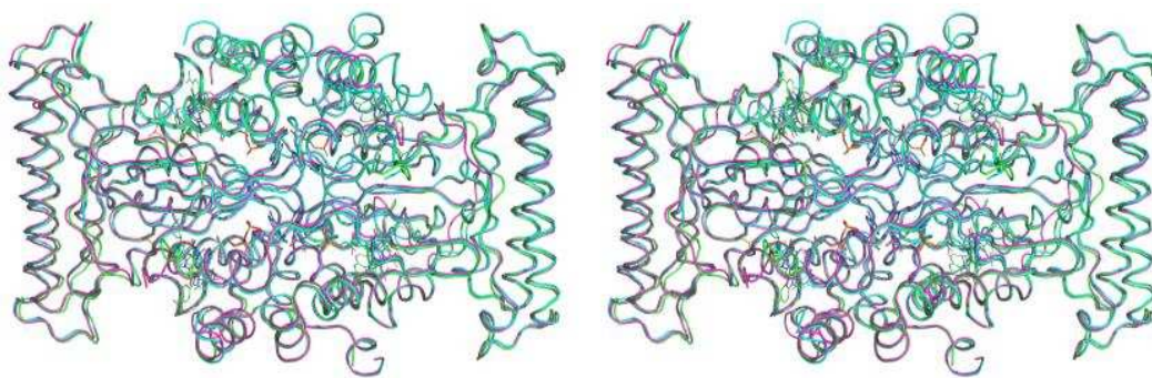
Supplementary Figure 8: Stereo-view of structural comparison of apoThyX/synthetic 4' (violet), FADH•CH 2 O (cyan) and ThyX in complex with CH 2 THF and dUMP (pdb, 4gt9, green).
