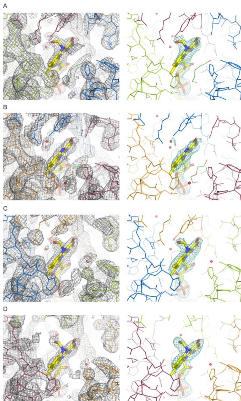
Supplementary Figure 9: Section of the 2mF_0 - DF_c electron density (left) and omit map (right) contoured at 1\sigma of the four flavin binding sites observed in the asymmetric unit of apoThyX/synthetic 4'. Chains A,B,C,D are colored in limon, orange, blue and brown respectively. Flavin is represented as yellow sticks.
