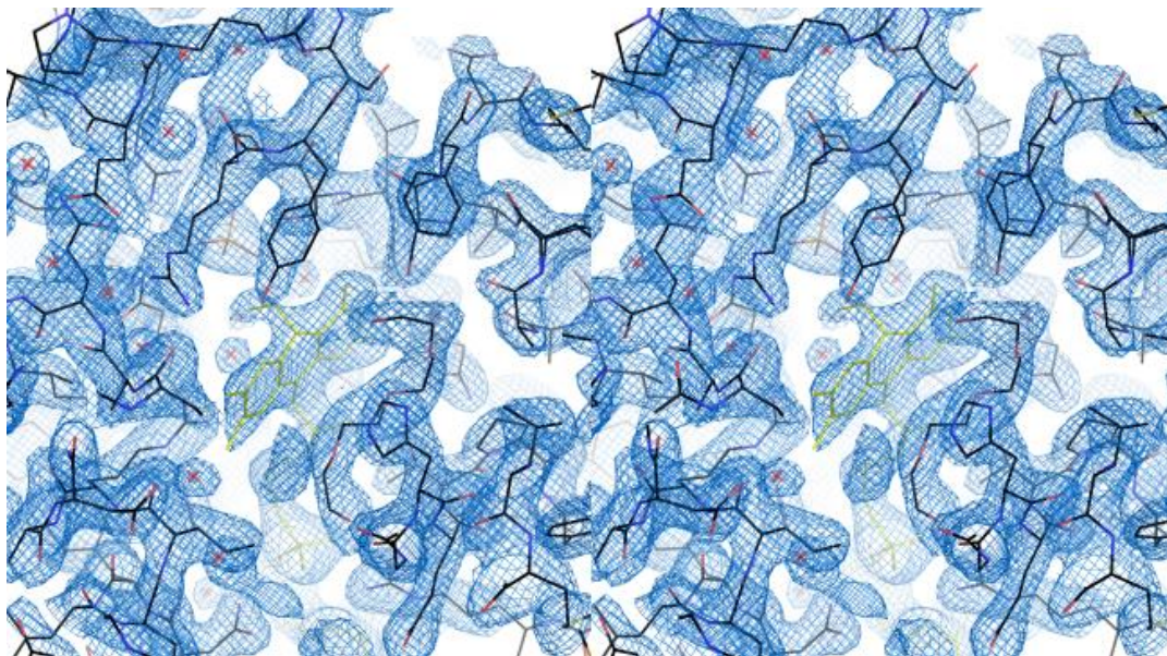
Supplementary Figure 11: Section of the electron density 2mF0-DFc contoured at the 1\sigma level around one 4' in the crystal of \text{FADH}^+\cdot\text{CH}_2\text{O} . The flavin is shown in yellow. For the protein C, N, O atoms are colored black, blue and red respectively.
