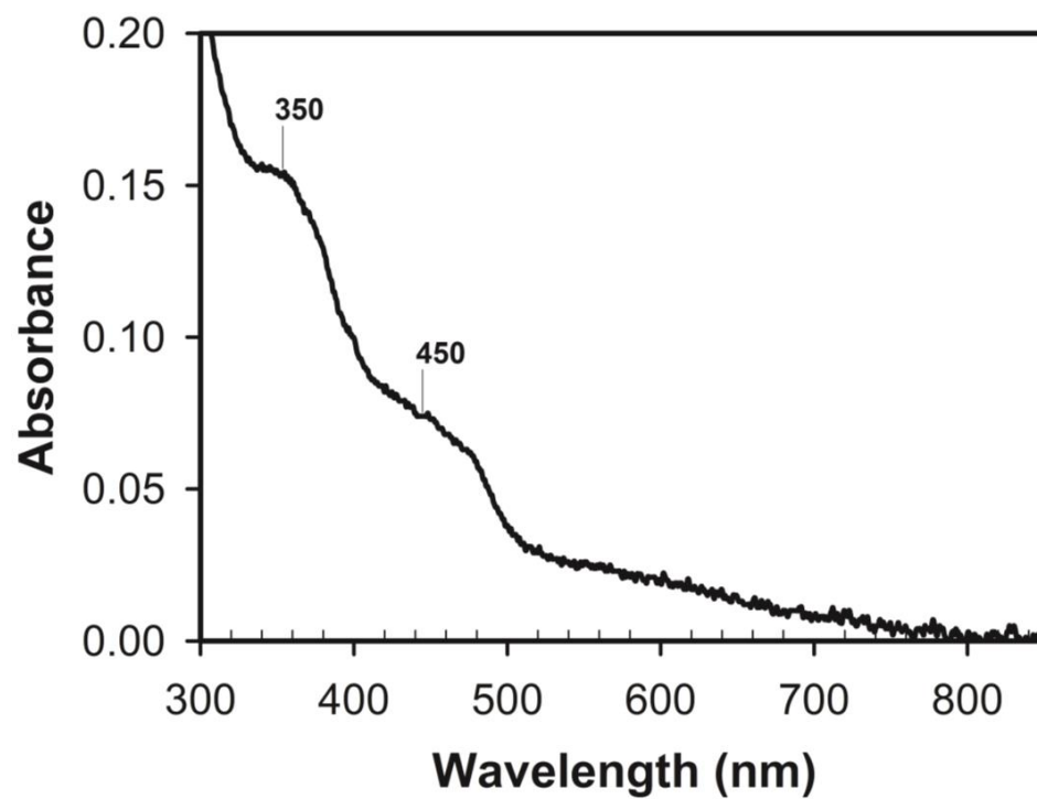
Supplementary Figure 7: Absorbance spectrum of crystal of ThyX in complex with the synthetic carbinolamine FAD derivative.
