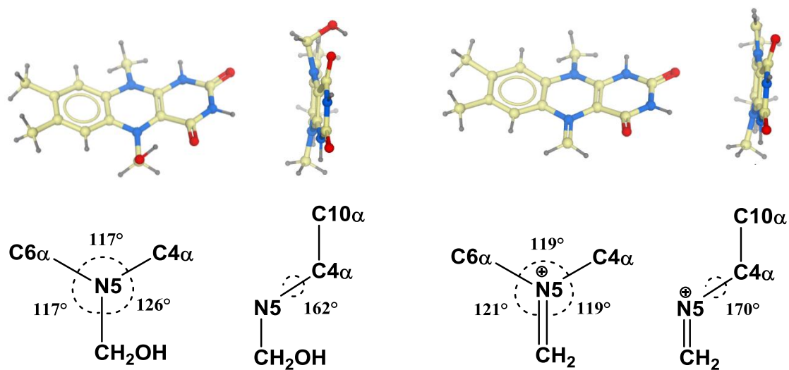
Supplementary Figure 14: Geometric comparison of a N5 carbinolamine and iminium flavin. a and b, 3D-model of N5-carbinolamine and N5-iminium adduct of lumiflavin in two different orientation, respectively. Below each model is shown the planar and torsion angles of each N5-adduct.
