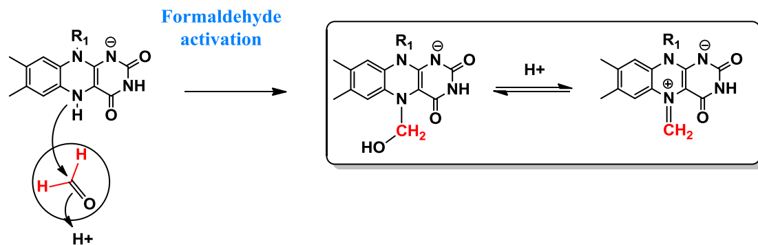
Supplementary Figure 2: Proposed mechanism for \text{CH}_2\text{O} activation by reduced FAD coenzyme. Nucleophilic N5 nitrogen of flavin hydroquinone, \text{FADH}^+ , attacks \text{CH}_2\text{O} to generate a carbinolamine flavin species, which in theory should be in equilibrium with its iminium counterpart. So far, the latter is postulated as being the bona fide dUMP methylating agent 2 .
