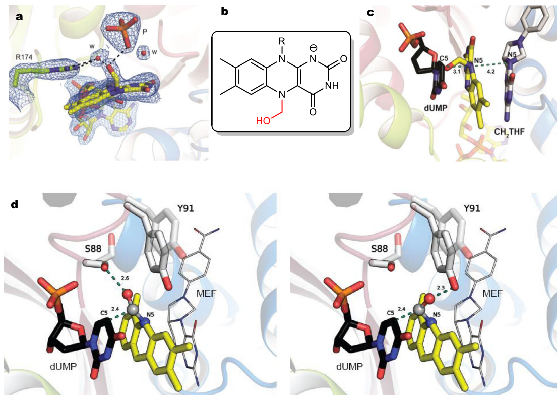
Fig. 3 Activation of \text{CH}_2\text{O} by T. maritima ThyX and structural capture of the carbinolamine flavin intermediate. a Section of the 2mF0-DFc electron density contoured at 1\sigma around the flavin carbinolamine of ThyX obtained by the anaerobic reaction of \text{CH}_2\text{O} with \text{FADH}^- ( \text{FADH}^- \cdot \text{CH}_2\text{O} ). Waters and a phosphate molecule are labeled w and P, respectively. R174 participates in dUMP activation 24 and interacts with an active site water molecule. b Chemical structure of the N5 flavin-carbinolamine adduct. c Model of ThyX in complex with the flavin carbinolamine, dUMP, and folate. The model was obtained by superimposing the crystal structure of \text{FADH}^- \cdot \text{CH}_2\text{O} complex with the structure of ThyX in complex with dUMP and folate (pdb, 4gt9). d Structural model of ThyX in complex with the flavin carbinolamine, dUMP, and folate, in which the carbinolamine is properly oriented for attack by the activated C5-dUMP. This \text{S}_\text{N}2 is likely assisted by two residues, S88 and Y91, which are conserved among ThyX enzymes. This model shows the different orientations adopted by these residues in two different structures of ThyX and they may assist the \text{S}_\text{N}2 and departure of the \beta -hydroxyl leaving group of the flavin carbinolamine. The structures used for this model are: (i) ThyX \text{FADH}^- soaked with 20 mM \text{CH}_2\text{O} vs (ii) pdb 4gt9.
