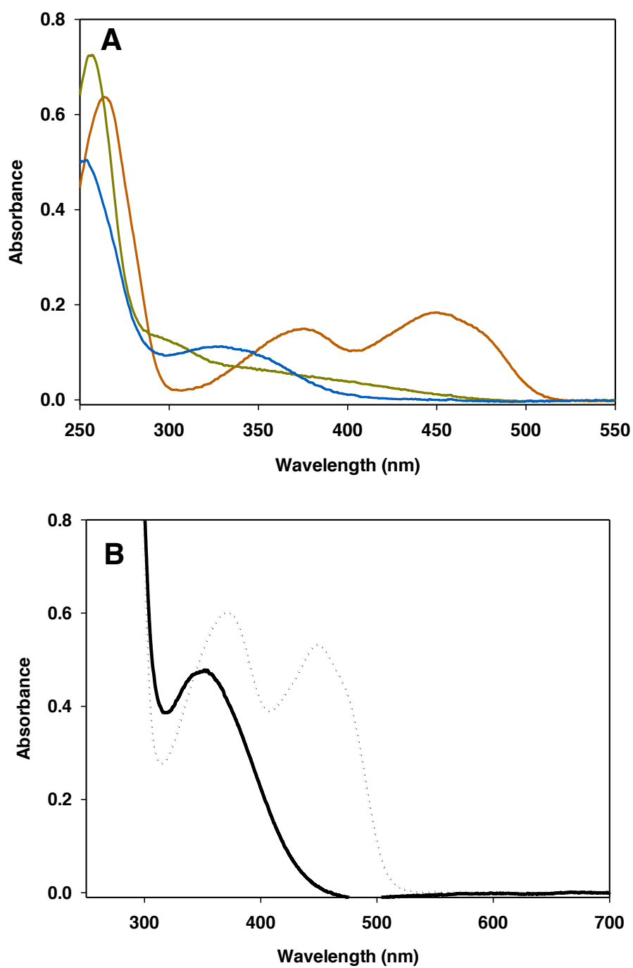
Supplementary Figure 6: Reaction of free reduced FAD with formaldehyde and reconstitution with apoThyX. A) Absorbance spectrum of 15 \mu\text{M} free FAD (orange), reduced FAD with 1 molar equivalent dithionite (green) or incubated with 100 mM \text{CH}_2\text{O} (blue). B) Absorption of reconstituted ApoThyX with the carbinolamine FAD adduct after PD-10 desalting column in the absence of dUMP (solid line) or in the presence of 1 mM dUMP (dotted line).
