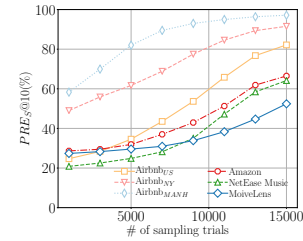
Figure 10: Impact of the number of sampling trails.
