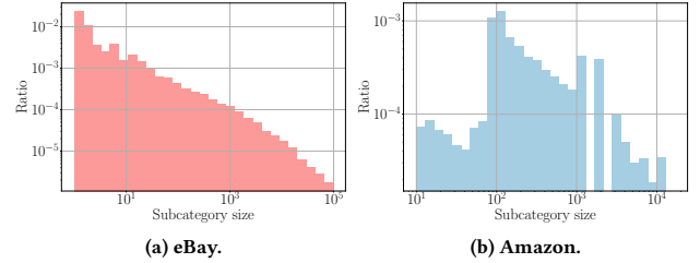
Figure 11: Distributions of subcategory size on eBay and Amazon.
