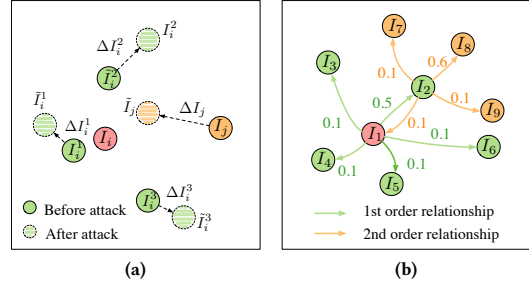
Figure 4: (a) Attacking item proximities by altering the item distributional representations. (b) Sampling items with first-order relationship or second-order relationship.
