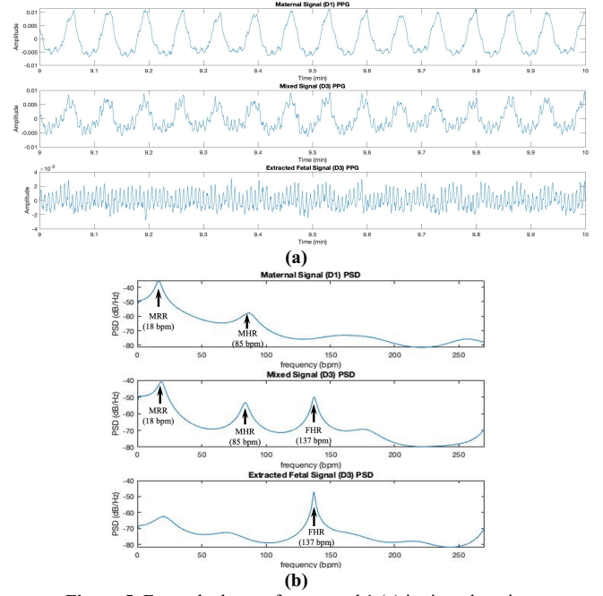
Figure 5. Example dataset from round 1 (a) in time-domain, (b) in frequency domain
