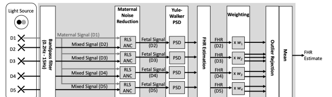
Figure 4. Multi-Detector Fetal Heart Rate Estimation Block Diagram
