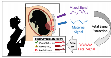
Figure 2. High-Level overview of Transabdominal Fetal Pulse Oximetry [16].
