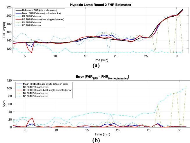
Figure 7. Hypoxic lamb round 2 results. (a) FHR estimates, (b) FHR estimation error over time
