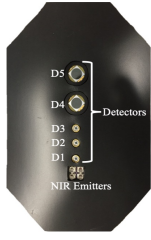
Figure 1. Optical Probe.
