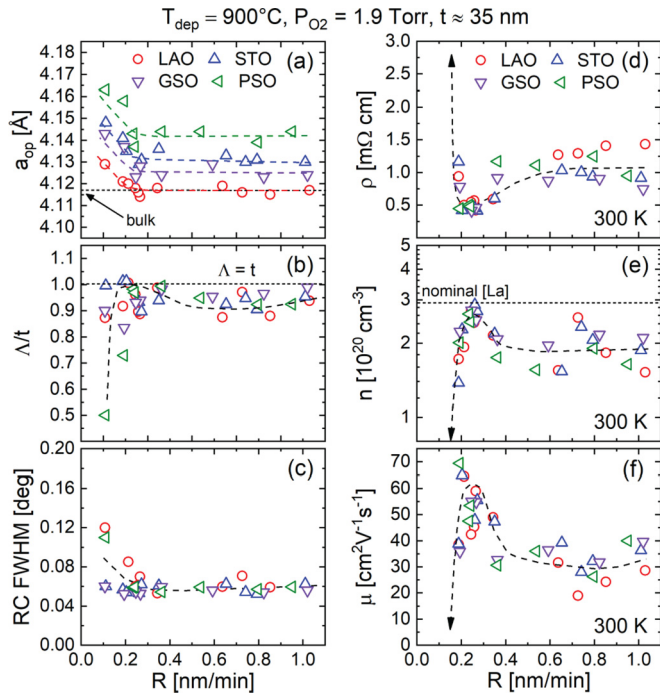
FIG. 9. Deposition rate ( R ) dependence of (a) the out-of-plane lattice parameter ( a_{op} ), (b) the Scherrer length-to-thickness ratio ( \Delta/t ), (c) the 002 rocking curve full width at half maximum (RC FWHM), (d) the 300 K resistivity ( \rho ), (e) the 300 K Hall electron density ( n ), and (f) the 300 K Hall mobility ( \mu ) for \text{La}_{0.02}\text{Ba}_{0.98}\text{SnO}_3 (BSO:La) films on \text{LaAlO}_3 (LAO), \text{SrTiO}_3 (STO), \text{GdScO}_3 (GSO), and \text{PrScO}_3 (PSO) substrates. The deposition temperature ( T_{\text{dep}} ), oxygen pressure ( P_{\text{O}_2} ), and thickness ( t ) were held constant at 900 °C, 1.9 Torr, and \sim 35 nm, respectively. The horizontal black dashed lines in (a), (b), and (e) mark the bulk lattice parameter \Lambda = t and the nominal n for full dopant activation, respectively. Colored dashed lines are guides to the eye. The arrows in the right panels indicate that lower R values resulted in much larger \rho , lower n , and lower \mu , off scale in (d) and (e).
