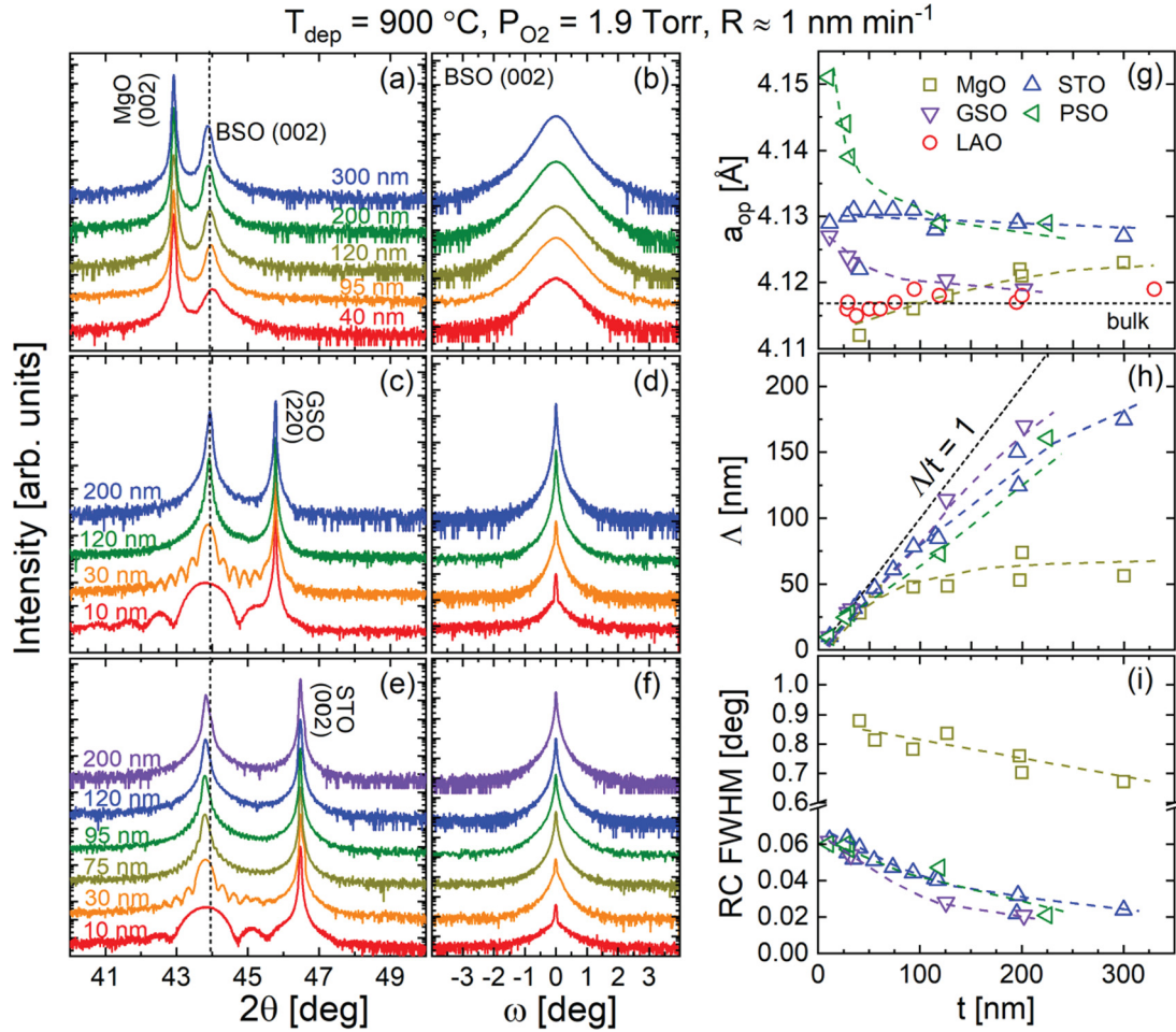
FIG. 4. (a), (c), and (e) High-resolution wide-angle specular x-ray diffraction around the 002 film and 002/220 substrate reflections and (b), (d), and (f) corresponding 002 film rocking curves, from \text{La}_{0.02}\text{Ba}_{0.98}\text{SnO}_3 (BSO:La) films with various thickness ( t ). Data are offset for clarity and are shown on MgO, GdScO 3 (GSO), and SrTiO 3 (STO) substrates. Deposition temperature ( T_{\text{dep}} ), oxygen pressure ( P_{\text{O}_2} ), and deposition rate ( R ) were held constant at 900^\circ\text{C} , 1.9 Torr, and \sim 1 nm min -1 , respectively. The vertical black dotted line in (a), (c), and (e) corresponds to the bulk lattice parameter. t dependence of (g) the out-of-plane lattice parameter ( a_{\text{op}} ), (h) the Scherrer length ( \Lambda ), and (i) the 002 film rocking curve full width at half maximum (RC FWHM) on MgO, STO, GSO, PrScO 3 (PSO), and LaAlO 3 (LAO) substrates (note the break on the RC FWHM axis). The black dotted lines in (g) and (h) mark the bulk lattice parameter and \Lambda = t , respectively. The colored dashed lines in (g), (h), and (i) are guides to the eye.
