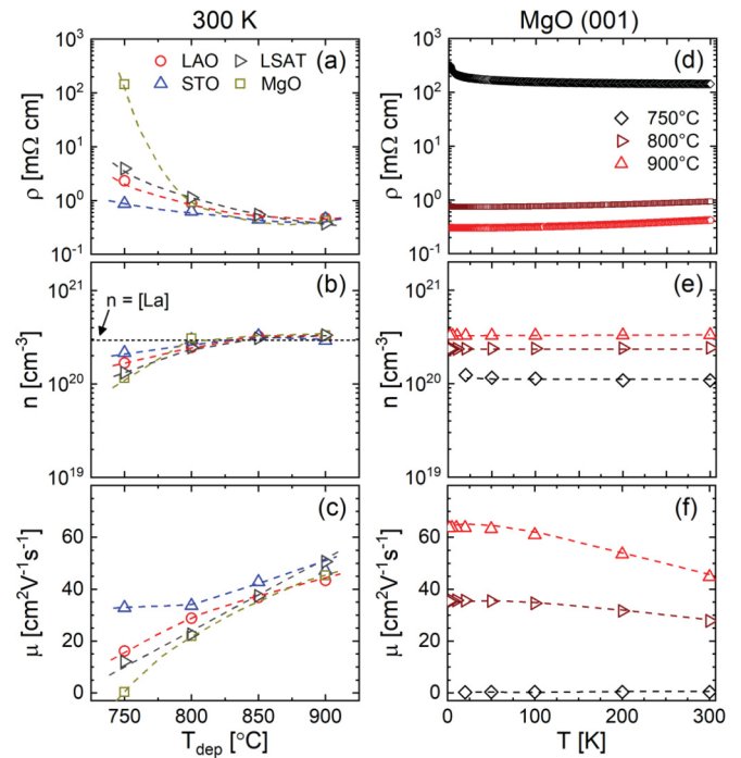
FIG. 3. Deposition temperature ( T_{\text{dep}} ) dependence of the 300 K (a) resistivity ( \rho ), (b) Hall electron density ( n ), and (c) Hall mobility ( \mu ) for \text{La}_{0.02}\text{Ba}_{0.98}\text{SnO}_3 (BSO:La) films on MgO, \text{LaAlO}_3 (LAO), \text{SrTiO}_3 (STO), and (\text{LaAlO}_3)_{0.3}(\text{Sr}_2\text{TaAlO}_6)_{0.7} (LSAT) substrates. Oxygen pressure, deposition rate, and thickness were held constant at 1.9 Torr, \sim 1 nm \text{min}^{-1} , and \sim 80 nm, respectively. Temperature dependence of (d) \rho , (e) n , and (f) \mu for the films on MgO in (a), (b), and (c), respectively. The horizontal black dotted line in (b) marks the nominal n for full dopant activation. Colored dashed lines are guides to the eye.
