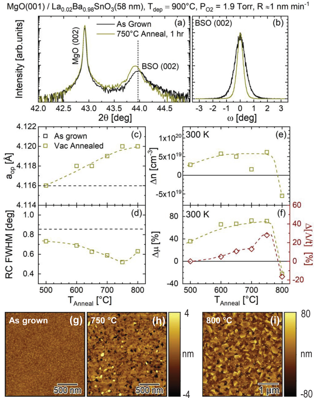
FIG. 10. (a) High-resolution wide-angle specular x-ray diffraction around the 002 film and substrate reflections and (b) corresponding 002 film rocking curves from a \text{La}_{0.02}\text{Ba}_{0.98}\text{SnO}_3 (BSO:La) film before and after vacuum annealing for 1 h at 750 °C. The vertical black dashed line in (a) corresponds to the bulk lattice parameter. All data in this figure are from films deposited on MgO at 900 °C, in 1.9 Torr of \text{O}_2 , at \sim 1 \text{ nm min}^{-1} , to \sim 58 \text{ nm} thickness. (c)–(f) Annealing temperature ( T_{\text{anneal}} ) dependence of (c) the out-of-plane lattice parameter ( a_{\text{op}} ), (d) the 002 film rocking curve full width at half maximum (RC FWHM), (e) the annealing-induced change in 300 K Hall electron density ( \Delta n ), and (f) the annealing-induced change in 300 K Hall mobility ( \Delta\mu ). Shown on the right axis in (f) is the annealing-induced change in Scherrer length-to-thickness ratio ( \Delta[\Delta/t] ). The horizontal black dashed lines in (c) and (d) represent average values for as-grown films; all other dashed lines are guides to the eye. Contact-mode atomic force microscopy (AFM) images of (g) an as-grown film, (h) a 750 °C annealed film, and (i) an 800 °C annealed film; scale bars are provided.
