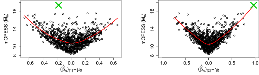
Figure 7: (Left) mOPeSS as a function of the of (\hat{\beta}_n)_{[1]} - \mu_0 (in this case \mu_0 = 0 ). (Right) mOPeSS (\bar{M}_n) as a function of (\hat{\beta}_n)_{[2]} - \gamma_0 (in this case \gamma_0 = 0 ). Each point corresponds to one of the 1,000 simulated datasets. The cross symbol indicates the maximum observed mOPeSS across all 1,000 simulation studies, \approx 19 .
