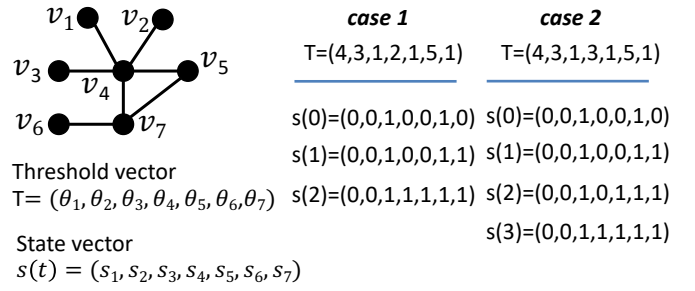
Fig. 1: Schematic of a GDS, showing a 7-node graph G , threshold vector T , and state vectors s(t) as they update over time. There are two cases, each involving a threshold vector T where the only difference between them is that \theta_4 increases from 2 to 3 for v_4 . These cases are discussed in the text.
