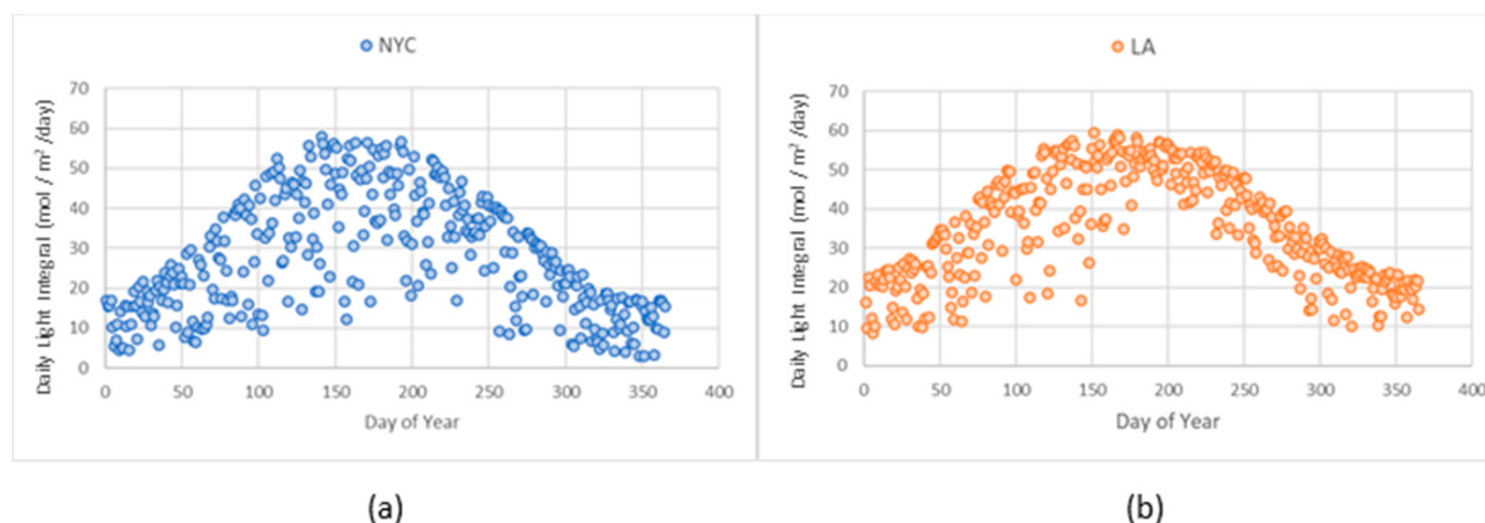
Figure 3. Daily light integral ( \text{mol} \cdot \text{m}^{-2} \cdot \text{day}^{-1} ) in (a) New York City and (b) Los Angeles.
