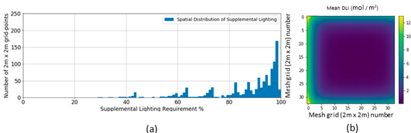
Figure 5. (a) Distribution of supplemental lighting requirements at 19th-level of Geometry 3 in New York and (b) map of mean DLI of natural light throughout building interior.
