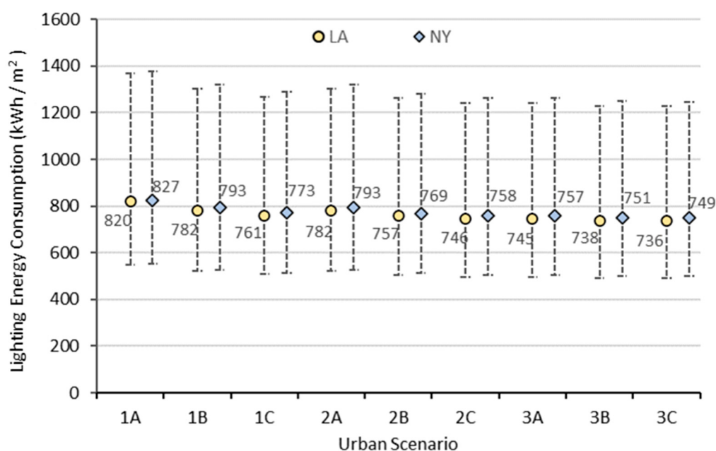
Figure 7. Annual lighting energy use index ( \text{kWh}\cdot\text{m}^{-2} ) of nine urban settings (described in Table 3) for New York (NY) and Los Angeles (LA). The error bars represent the lighting energy consumption for different assumptions using PAR efficacy of 3\ \mu\text{mol}\cdot\text{J}^{-1} (lower bar) and 1.2\ \mu\text{mol}\cdot\text{J}^{-1} (upper bar).
