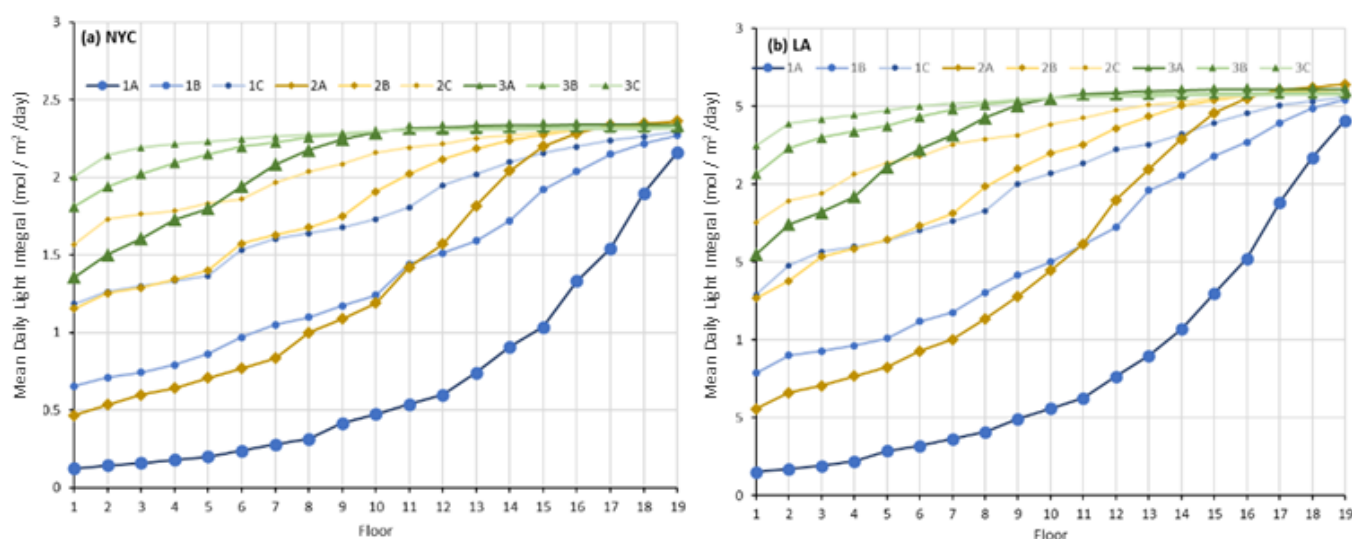
Figure 6. Mean daily light integral (DLI) ( \text{mol} \cdot \text{m}^{-2} \cdot \text{day}^{-1} ) for each level of a skyscraper farm in NYC (a) and LA (b) under different urban scenarios. Details of urban scenarios are described in Table 2.
