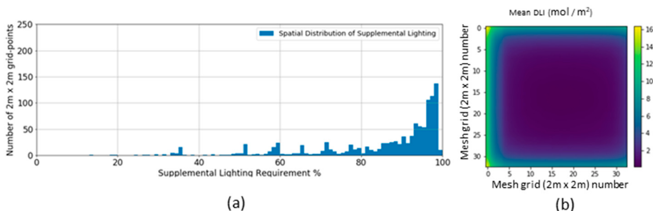
Figure 4. (a) Distribution of supplemental lighting requirements at 19th level of Geometry 3 in Los Angeles and (b) map of mean DLI of natural light throughout building interior.
