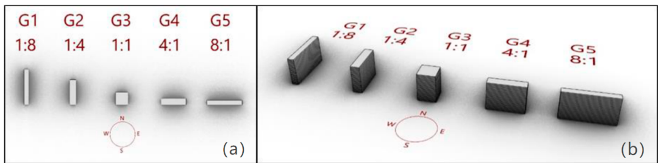
Figure 1. (a) Top-view and (b) perspective view of skyscraper farm geometries G1–G5 with corresponding side ratios. All buildings had 20 floors with 5 m inter-floor height.
