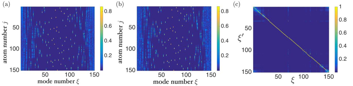
FIG. 3. A representative plot of the excitation amplitude |c_j^\xi| versus atom number j and eigenmode index \xi , for a single disorder realization and within the single-excitation manifold. The excitation amplitudes are plotted for (a) the effective non-Hermitian Hamiltonian \mathcal{H}_{\text{ID}} and (b) its Hermitian component \mathcal{H}_{\text{hermi}} . (c) Magnitude of the dot product between the eigenmodes of the two Hamiltonians: D(\xi, \xi') = |\langle \psi_\xi^{(\text{ID})} | \psi_{\xi'}^{(\text{hermi})} \rangle| . All of these plots were generated for a system of N = 150 atoms.
