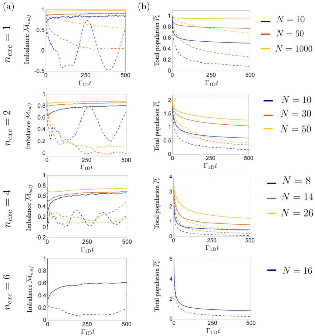
FIG. 8. Time-dependent, disorder-averaged population imbalance \overline{M}_{half}(t) (a) and total population \overline{P}_e(t) (b) for the open half-waveguide, for n_{exc} = 1, 2, 4, 6 initial excitations, and for various system sizes N (indicated by different colors). We plot these quantities both for the disordered (solid curves) and ordered (dashed) systems.
