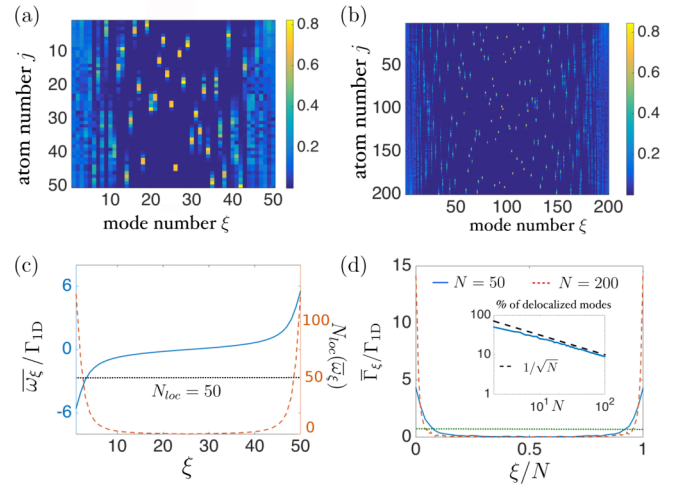
FIG. 2. Spatial profile of the single-excitation eigenmodes |c_j^\xi| of the effective Hamiltonian \mathcal{H}_{1D} , ordered with respect to the real part of their eigenvalue, for two different system sizes: N = 50 (a) and N = 200 (b). These eigenmodes have been calculated for a single disorder realization, and are indexed from lowest ( \xi = 1 ) to highest ( \xi = N ) frequency. (c) Average value over a large number of disorder realizations of \omega_\xi/\Gamma_{1D} (solid blue line) as a function of \xi , together with the associated Anderson localization length N_{\text{loc}}(\omega_\xi) (dashed orange line) in units of number of atoms. This plot is calculated for N = 50 atoms. For reference, we indicate where the localization length corresponds to the system size by the dotted black line. (d) Average value over a large number of disorder realizations of the normalized decay rate \Gamma_\xi/\Gamma_{1D} of eigenmodes, as a function of \xi/N , for two different system sizes N = 50 (solid blue line) and N = 200 (dashed orange line). A large fraction of modes have a decay rate smaller than \Gamma_{1D}/2 (dotted green line). Numerically, the percentage of modes with decay rate larger than \Gamma_{1D}/2 decreases approximately as \sim 1/\sqrt{N} (inset).
