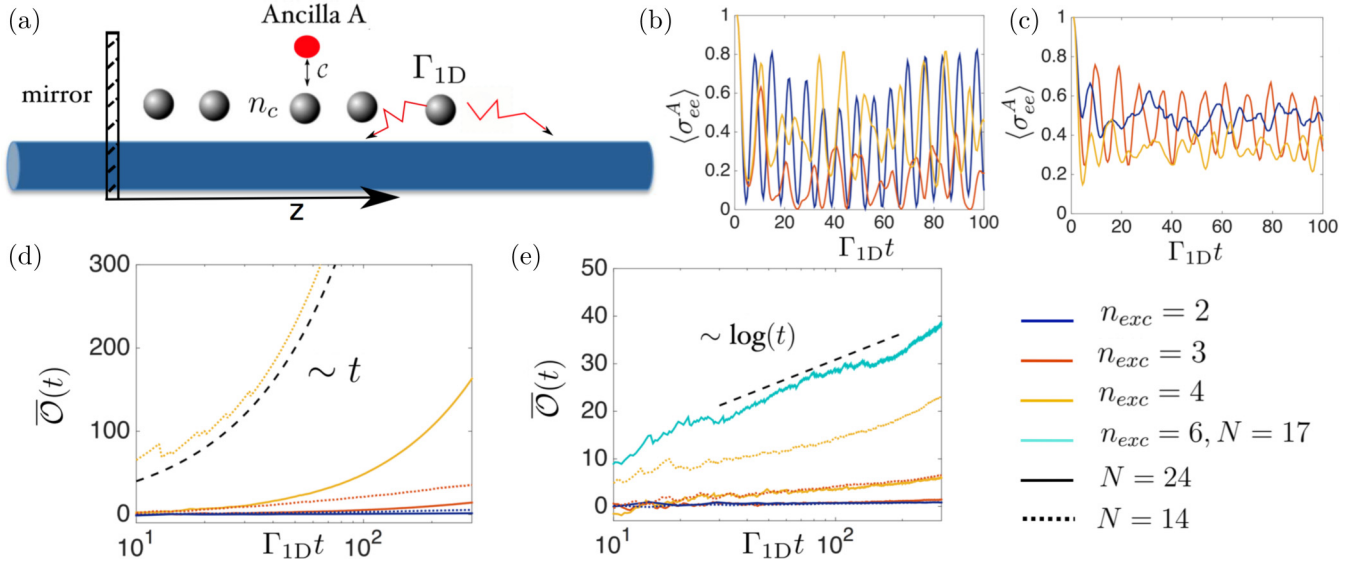
FIG. 9. (a) Scheme of the quantum revival setup to measure the interacting degrees of freedom in the open half-waveguide. An additional ancilla A is introduced, which does not couple or radiate into the waveguide, but couples to and can exchange excitations with the waveguide atom n_c . The time-dependent excited population of the ancilla is monitored to record the number of revivals N_{\text{rev}} within a certain time window [0, t] . [(b) and (c)] Ancilla population versus time, for three typical disorder realizations for a Hermitian half-waveguide. Here initially the ancilla is excited, while the waveguide atoms contain no excitations (b) and 2 excitations located at positions |e_1, e_4\rangle (c). The total system size (ancilla + atoms) is N = 14 . Disorder-averaged \bar{\mathcal{O}}(t) for both Hermitian (d) and open (e) disordered systems of size N = 14 (dotted curves), N = 17 (light blue curve), and N = 24 (solid curves) with varying number of excitations ( n_{\text{exc}} = 2, 3, 4, 6 ) indicated by different colors. As a guide to the eye, we show a linear evolution in (d) and a logarithmic evolution in (e) in black dashed curves.
