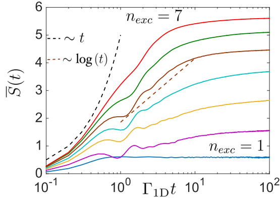
FIG. 7. Disorder-averaged half-chain entanglement entropy \bar{S}(t) as a function of time, for different number of atomic excitations initially prepared in a product state, in the Hermitian waveguide. The simulations are for N = 20 atoms, and the curves from bottom to top correspond to 1 \leq n_{\text{exc}} \leq 7 excitations. Linear and logarithmic scalings (dashed curves) are shown as a guide to the eye.
