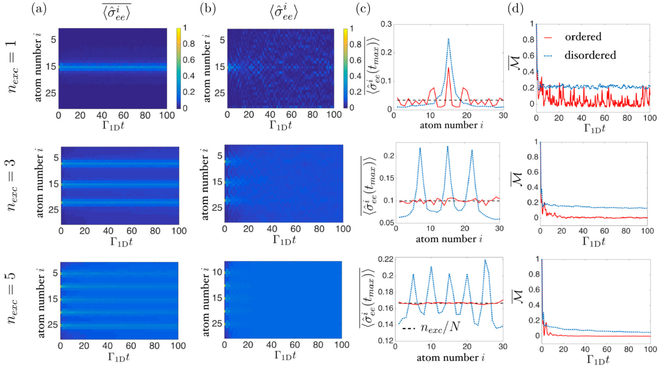
FIG. 4. Transport properties of N = 30 atoms in the Hermitian waveguide, averaged over disorder configurations. Each line corresponds to a different number of excitations ( n_{\text{exc}} = 1, 3, 5 ), initialized in a product state. In (a) and (b), we plot the time-dependent, site-resolved excited-state population \langle \hat{\sigma}_{ee}^i(t) \rangle , for disordered and ordered systems, respectively. (c) Site-resolved population \langle \hat{\sigma}_{ee}^i(t_{\max}) \rangle evaluated at the final simulation time t_{\max} = 100/\Gamma_{1D} , for both disordered (blue dotted line) and ordered systems (solid red line). As a guide to the eye, we plot n_{\text{exc}}/N (dashed line), the population if the initial excitations were to become uniformly distributed. (d) Time-dependent memory parameter \mathcal{M}(t) for both disordered (blue dotted line) and ordered systems (solid red line).
