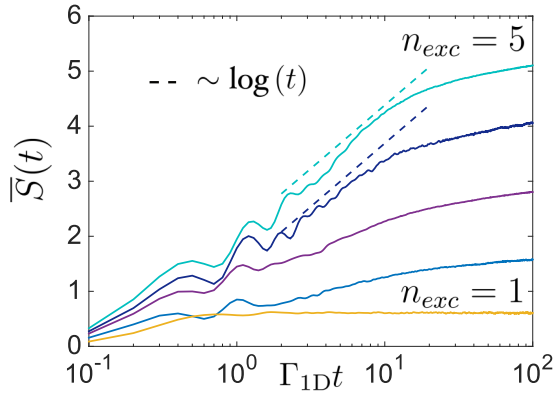
FIG. 5. Disorder-averaged half-chain entanglement entropy \bar{S}(t) as a function of time, for different number of atomic excitations initially prepared in a product state, in the Hermitian waveguide. The simulations are for N = 30 atoms, and the curves from bottom to top correspond to 1 \leq n_{\text{exc}} \leq 5 excitations. Logarithmic scalings (dashed lines) are shown as a guide to the eye.
