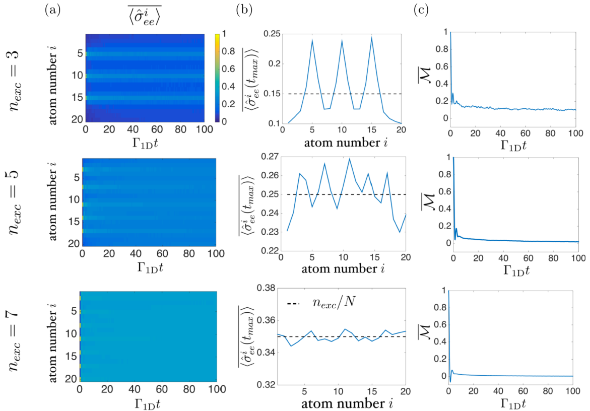
FIG. 6. Transport properties of N = 20 atoms in the Hermitian waveguide, averaged over disorder configurations. Each line corresponds to a different number of excitations ( n_{\text{exc}} = 3, 5, 7 ), initialized in a product state. (a) Time-dependent, site-resolved excited-state population \langle \hat{\sigma}_{ee}^i(t) \rangle . (b) Site-resolved excited-state population at the final simulation time, t_{\text{max}} = 100/\Gamma_{1D} . As a guide to the eye, we plot n_{\text{exc}}/N (dashed line) to indicate the population if the excitations become equally distributed. (c) Time-dependent memory parameter \bar{\mathcal{M}}(t) .
