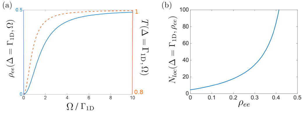
FIG. 10. (a) Excited-state population \rho_{ee} (blue solid line) and transmittance T of a single atom (orange dashed line) as a function of driving Rabi amplitude \Omega/\Gamma_{1D} and at a detuning \Delta = \Gamma_{1D} . (b) The estimated MBL localization length N_{loc}(\Delta = \Gamma_{1D}, \rho_{ee}) as a function of atomic population.
