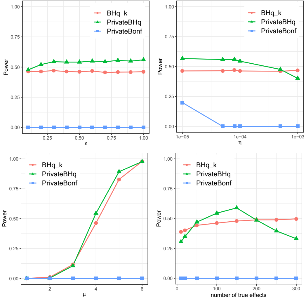
FIGURE 5. The power of BHq_k , PrivateBHq, and PrivateBonf, plotted against varying \epsilon, \eta, \mu, m_1 , respectively, and averaged over 100 independent replicates.
