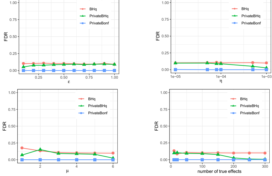
FIGURE 2. The FDR of BHq, PrivateBHq, and PrivateBonf, plotted against varying \varepsilon, \eta, \mu, m_1 , respectively, and averaged over 100 independent replicates. Note that PrivateBHq in general discovers fewer than BHq and has a smaller FDR than BHq as well.
