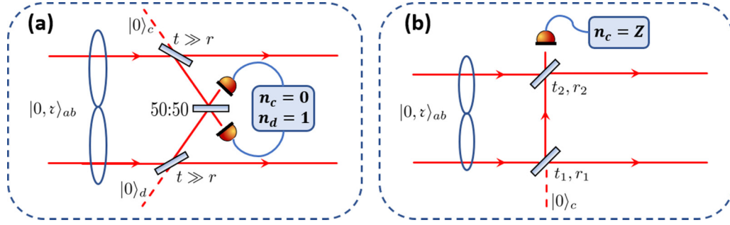
FIG. 2. (a) Scheme using two click detectors to indistinguishably subtract a single photon from two squeezed modes. (b) Simplified version using a single detector that includes the case of coherent single-photon subtraction, but also extends the method to include coherent Z -photon subtraction when a PNR detector is used.
