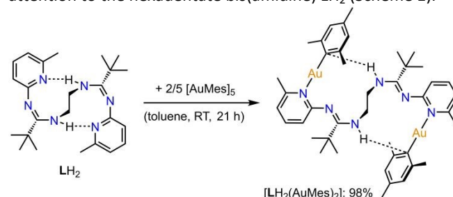
Scheme 1 Synthesis of complex [LH 2 (AuMes) 2 ].
