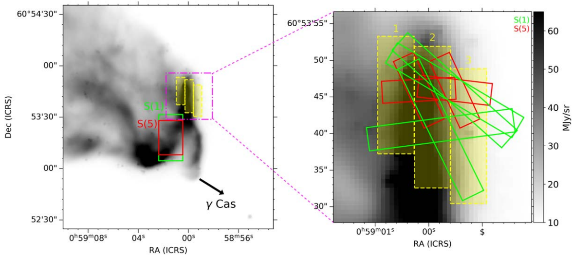
Figure 1. Left panel shows the location of the ISO/SWS slits and the three EXES regions over an 8.0 \mu\text{m} Spitzer IRAC image (taken from Spitzer archive). The larger solid green rectangle is the ISO/SWS S(1) ( 17.0 \mu\text{m} ) aperture and the red solid rectangle is the S(5) ( 6.9 \mu\text{m} ) aperture (Thi et al. 2009). The purple dotted–dashed line shows the zoomed-in image in the right panel and the yellow rectangles show the three regions observed by SOFIA/EXES. The direction to \gamma Cas is shown as well. The right panel shows the zoomed-in view of the three extraction regions and the EXES slit positions over the 8.0 \mu\text{m} IRAC image. The SOFIA/EXES S(1) aperture is the larger solid green rectangles and the S(5) aperture is the smaller solid red rectangles. The slits swept clockwise during observations. We have defined region 1 as shady, region 2 as ridge, and region 3 as sunny and they are shown as translucent yellow rectangles.
