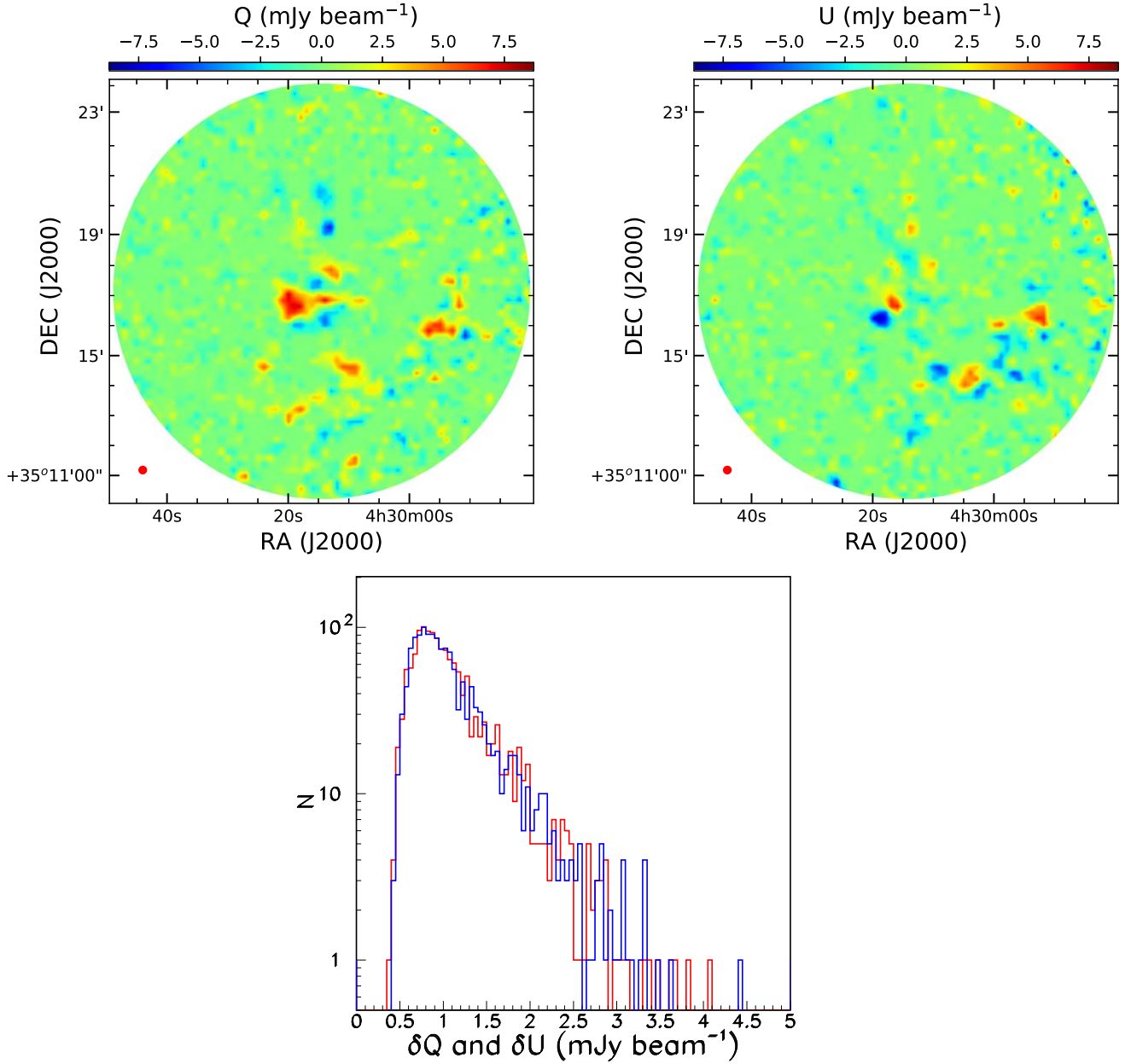
Figure 2. Upper: Q (left) and U (right) maps; the red circles at the lower-left corners indicate the JCMT beam size at 850\ \mu\text{m} of 14'' . Lower: distributions of \delta Q (red) and \delta U (blue).
