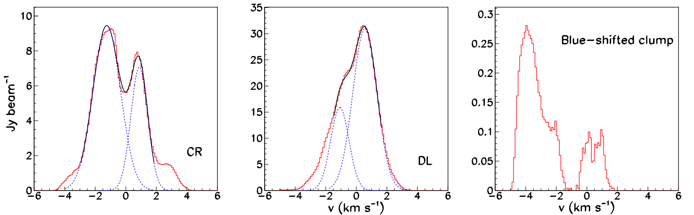
Figure 11. HARP CO(3–2) integrated spectra. Left: central region; center: dust lane. Right: blueshifted clump at RA \sim 4^{\text{h}}30^{\text{m}}07^{\text{s}} and decl. \sim +35^{\circ}13'20''5 . The blue dashed curves are the Gaussian components shown separately. The black curves are the results of the two-Gaussian fits (see text in Section 3.5).
