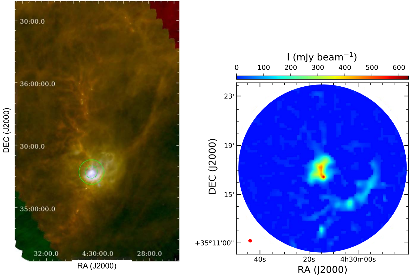
Figure 1. Left: the LkHα 101 field observed by POL-2 overlaid on the Herschel RGB image ( R = 250 \mu\text{m} , G = 160 \mu\text{m} , B = 70 \mu\text{m} ; Harvey et al. 2013). The green outer circle represents the 6' radius field of POL-2 and the green inner circle indicates the inner 3' radius with the best sensitivity. Right: 850 \mu\text{m} intensity map. The red circle at the lower-left corner of the panel shows the JCMT 850 \mu\text{m} beam size of 14".
