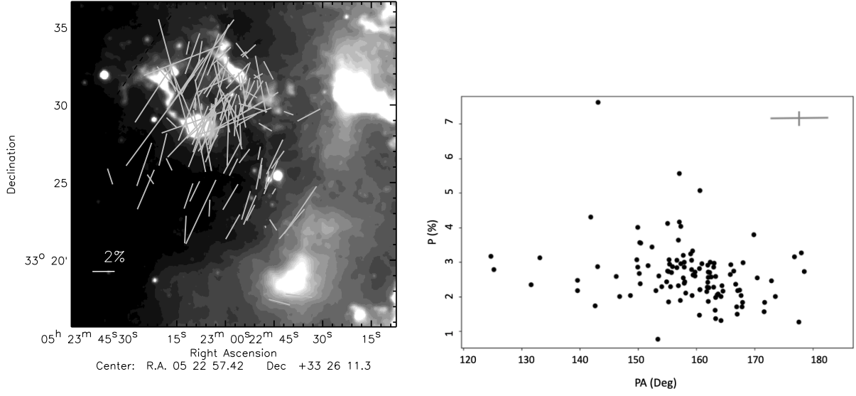
Fig. 1 Left panel: The polarization vectors plotted after correcting for the interstellar polarization. Right panel: The P vs. \theta_P distribution of measurements. A symbol signifying typical errors in P and \theta_P values is also marked.
