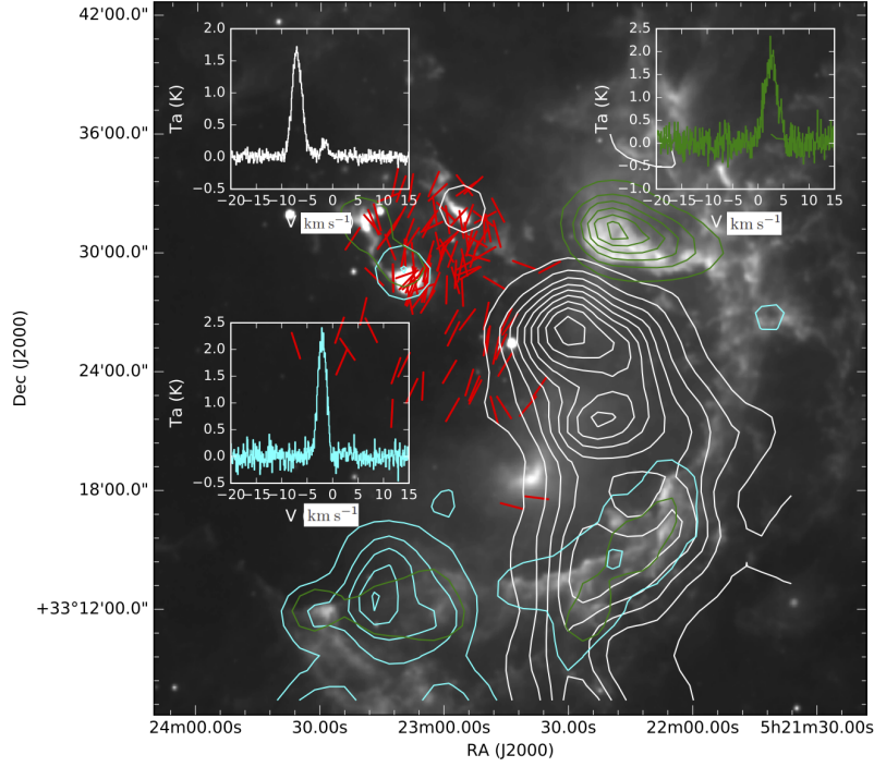
Fig. 5 WISE 12 \mu\text{m} image of NGC 1893 with overplotted CO (J=1–0) integrated intensity contours corresponding to three velocity components with V_{\text{LSR}} -7.0 \text{ km s}^{-1} (white), -2.5 \text{ km s}^{-1} (cyan) and V_{\text{LSR}} 2.5 \text{ km s}^{-1} (green) in the line of sight. The average spectra corresponding to these emissions are featured in the insets. The x axes of the insets represent the velocity and the y axes signify the antenna temperature. The red segments are normalized polarization vectors (independent of polarization fraction) illustrating the magnetic field morphology in this region.
