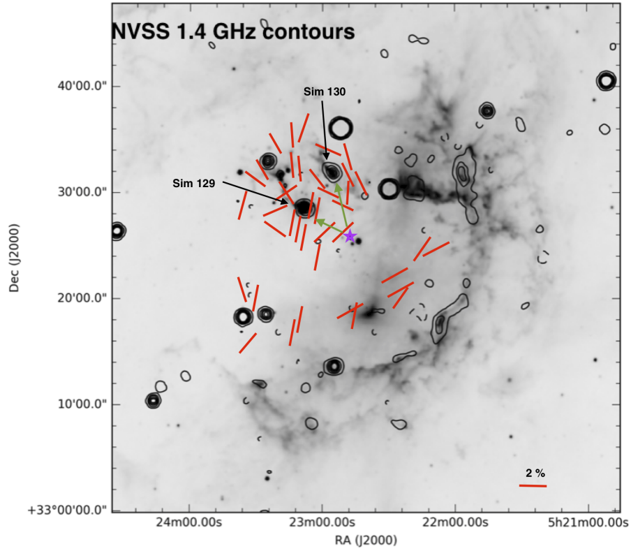
Fig. 8 Same as Fig. 4 with magnetic fields signified using normalized polarization vectors overplotted. The magenta star symbol marks the position of ionizing source HD 242935. The plane of the sky directions for ionizing radiation toward nebulae are illustrated with green vectors.
