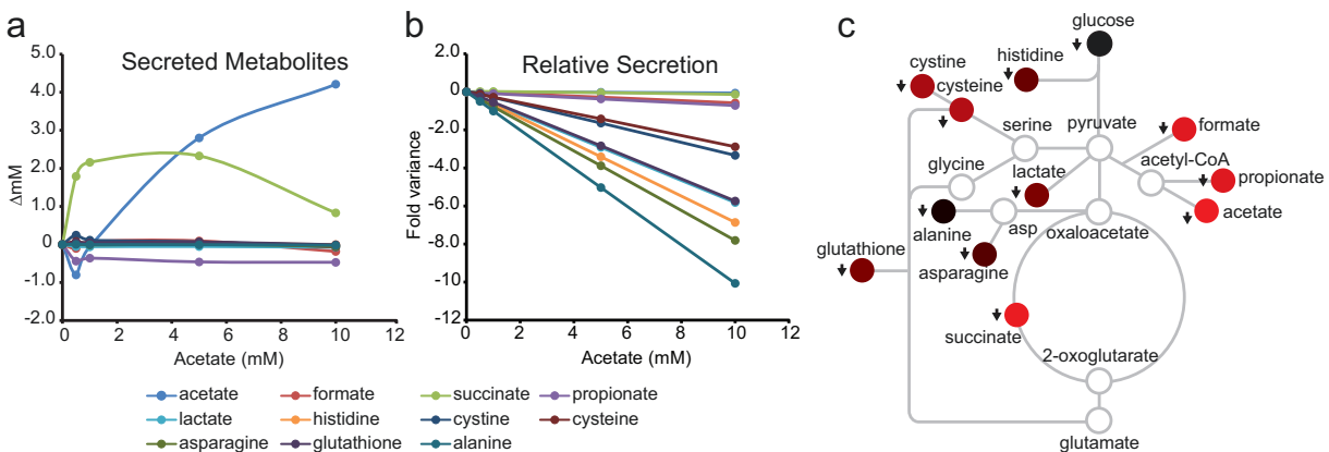
FIG 4 Effect of acetate feedback inhibition on secretion fluxes. (a) Concentrations of secreted metabolites with increasing acetate supplementation (means from 5 biological and 5 technical replicates, n = 25). P values are shown in Table S2. Error bars may be obscured by symbols. (b) Change in secretion fluxes with increasing acetate supplementation (means from 5 biological and 5 technical replicates, n = 25). P values are shown in Table S3. (c) Effect of acetate feedback inhibition (10 mM) mapped onto a metabolic network. Red, decreased secretion. Shading is proportional to flux magnitude. Gray outlined circles represent undetected intracellular metabolic nodes. asp, aspartate.
