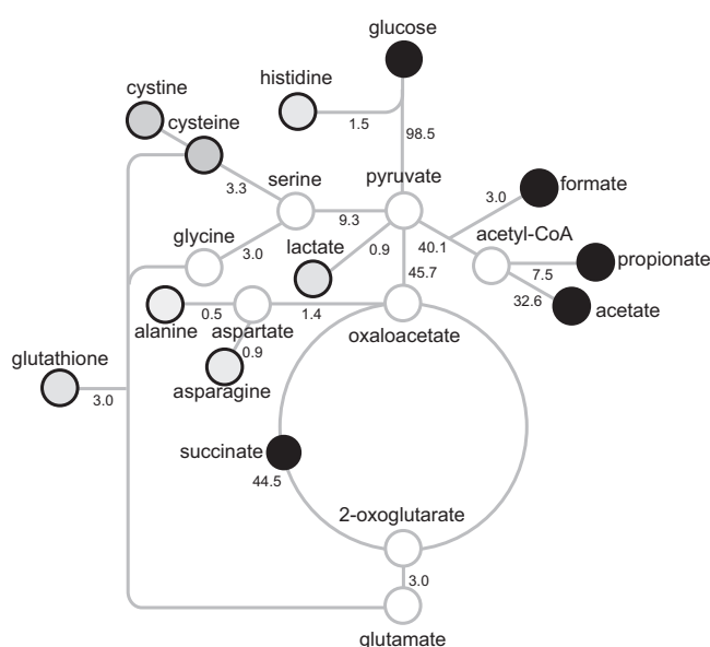
FIG 2 Secretion fluxes of organic acids and amino acids in defined minimal medium. Numbers represent percent mole carbon fluxes (not shown, \text{CO}_2 inferred, 4.6%). Gray outlined circles represent undetected intracellular metabolic nodes. Black outlined circles indicate secreted metabolites. Shading is proportional to concentration in culture medium.
