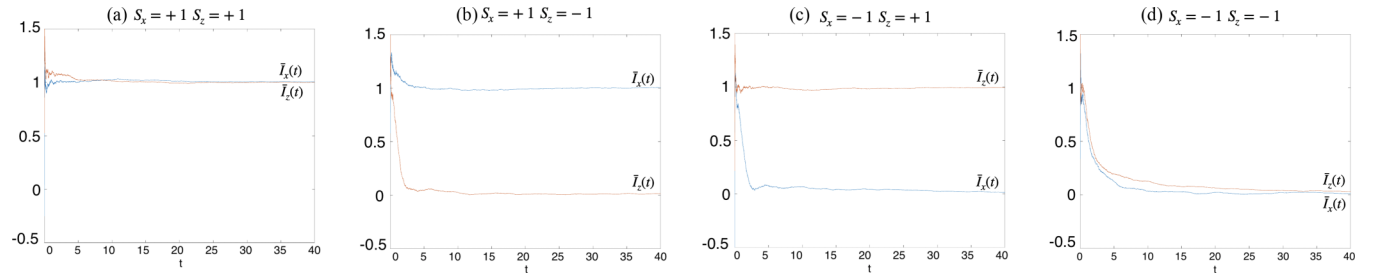
FIG. 2. \bar{I}_{x,z} verse time for the four eigenspaces. The red is \bar{I}_z(t) and the blue is \bar{I}_x(t) . The average function converges to 1 (or 0) if the corresponding stabilizer is in the +1 (or -1) eigenspace.
