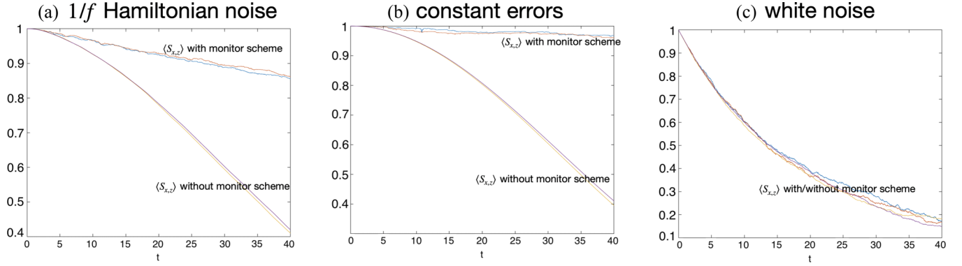
FIG. 7. The evolutions of the stabilizers under various error models. (a) compares evolutions of \langle S_{x,z} \rangle with/without indirect detection, under 1/f Hamiltonian noise. (b) compares evolutions of \langle S_{x,z} \rangle with/without indirect detection, under constant Hamiltonian errors. (c) is the case for white noise, where there shows no suppression of error. They are ensemble averages over 1000 trajectories.
