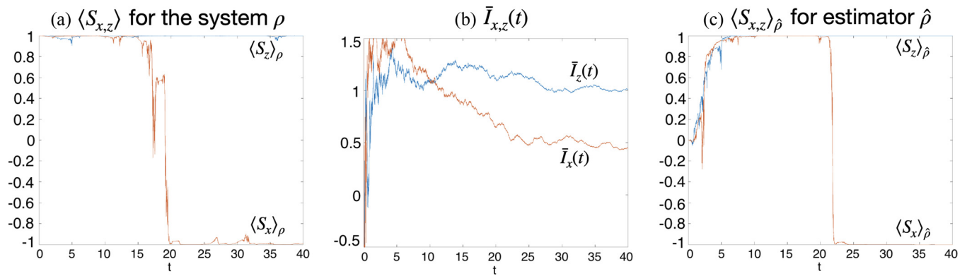
FIG. 5. (a) shows \langle S_{z,x} \rangle for the system. After a period, S_x is flipped to -1 while S_z remains at +1 . (b) shows \bar{I}_{x,z}(t) . After a period, \bar{I}_{z,x}(t) starts to decay while \bar{I}_z(t) remains at +1 . (c) shows \langle S_{z,x} \rangle_{\hat{\rho}} for the estimator. \langle S_x \rangle_{\hat{\rho}} approaches +1 initially, but it flips to -1 after \langle S_x \rangle \rightarrow -1 .
