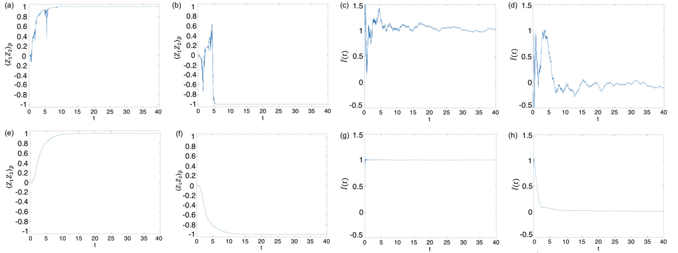
FIG. 1. (a), (b), (e), and (f) are the estimator approach. Each of (a) and (b) is a sample trajectory, and each of (e) and (f) is an ensemble average over 500 trajectories. The signals from measuring the physical state drive the estimator to the Z_1 Z_2 = \pm 1 eigenspace the physical state is in. (a) and (e) are the evolutions of \langle Z_1 Z_2 \rangle_{\hat{\rho}} when \rho is in the +1 eigenspace of Z_1 Z_2 . (b) and (f) are the cases when \rho is in the -1 eigenspace of Z_1 Z_2 . (c), (d), (g), and (h) represent the average function \bar{f}(t) . Each of (c) and (d) is a sample trajectory, and each of (g) and (h) is an ensemble average over 500 trajectories. It converges to 1 when the physical state is in the +1 eigenspace, and it converges to 0 when the state is in the -1 eigenspace.
