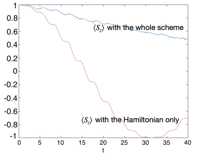
FIG. 9. The evolution of \langle S_z \rangle under an on-resonance X_1 error. The blue curve is the case when the full indirect detection scheme is applied. The red curve is the case when the Hamiltonian for indirect detection is applied but no measurements are made on the monitor qubits.
