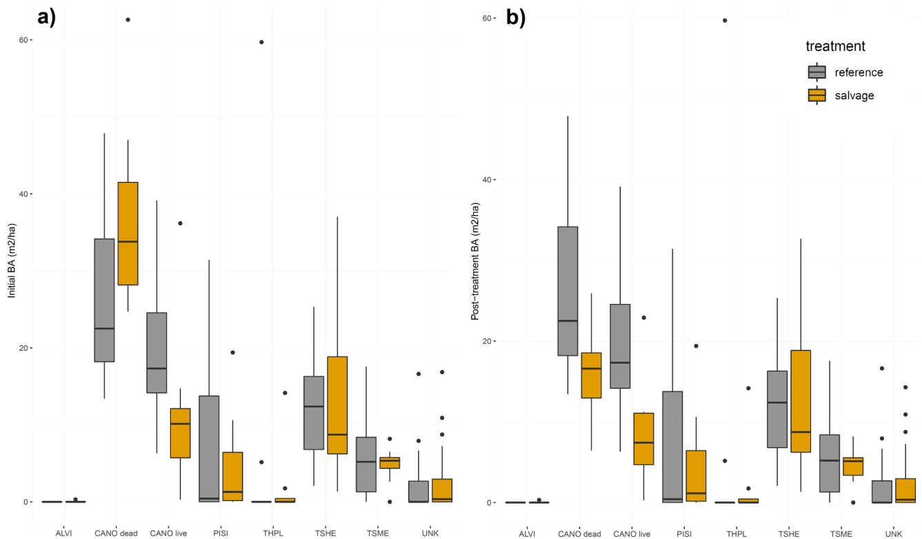
Fig. 2. Basal area ( \text{m}^2/\text{ha} ) by species and treatment. Total basal area (live and dead) is presented for each species with the exception of yellow-cedar ( \text{CANO} = \text{Callitropsis nootkatensis} ), which is separated into live vs. dead to illustrate the impact of the salvage operation on dead yellow-cedar canopy abundance. a) Pre-harvest basal areas were equivalent by species. b) Post treatment, salvage plots had a substantial decline in CANO basal area driven by salvage of dead CANO, but little to no change in the other species. Species acronyms are as follows - ALVI: Alnus viridis ; PISI: Picea sitchensis ; THPL: Thuja plicata ; TSHE: Tsuga heterophylla ; TSME: Tsuga mertensiana ; UNK: Unknown. (For interpretation of the references to colour in this figure legend, the reader is referred to the web version of this article.)
