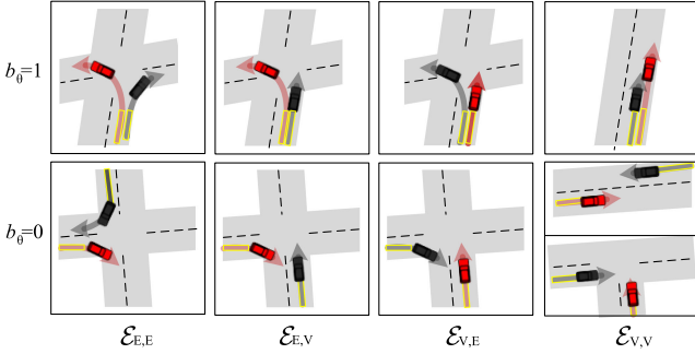
Fig. 4. Rendezvous events with same/different heading ( b_\theta ) which we use to identify vehicle relative locations. The yellow rectangular boxes mark out the latest vehicle stable headings used to determine b_\theta .
