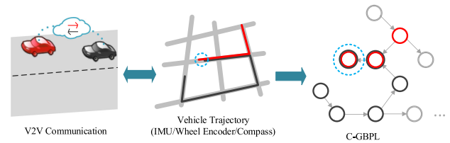
Fig. 1. An illustration of C-GBPL method using a two-vehicle rendezvous case. The ego vehicle is colored in red and the other vehicle is in black. At rendezvous, we aggregate vehicle trajectories to form a merged feature graph to facilitate localization.
