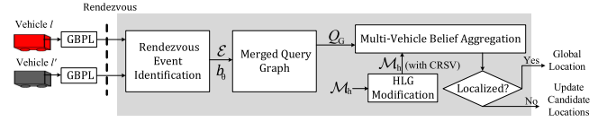
Fig. 2. C-GBPL system diagram.
