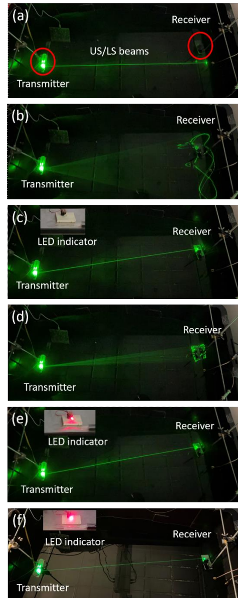
Figure 10. Photos showing the major operation steps of the searching, aiming and handshaking experiment: (a) Start pose. (b) Full-range searching. (c)
