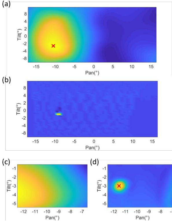
Figure 9. Reconstructed signal peak distribution map of (a) full-range ultrasound scan, (b) full-range laser scan, (c) fine-range ultrasound scan, and (d) fine-range laser scan. The red “x” signs represent the center of signal peak.
