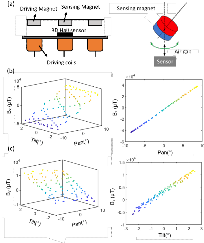
Figure 6. (a) Schematic diagram of the scan pose sensor. (b) Pose sensor reading ( B_x ) at different Pan and Tilt angles. (c) Pose sensor reading ( B_y ) at different Pan and Tilt angles.
