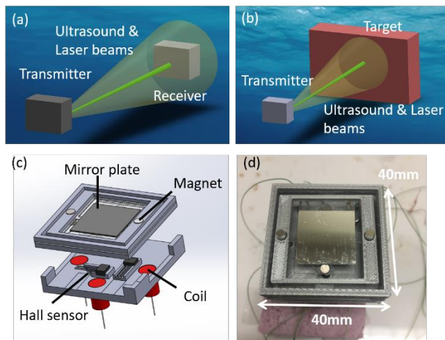
Figure 1. Illustration of the dual-modal scanning and aiming system for (a) communication and (b) ranging. (c) The schematic design and (d) photo of the previous WIMSM prototype [9].
