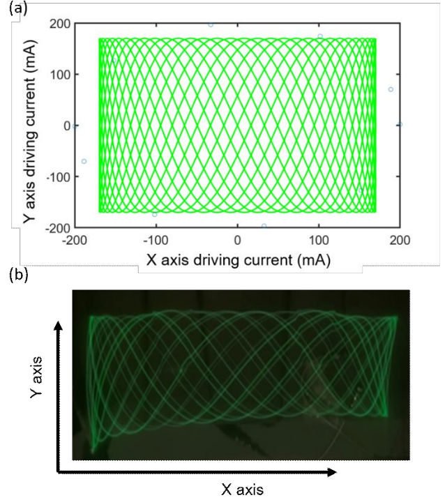
Figure 5. (a) The driving signals and (b) the scanning pattern of WIMSM under water.
