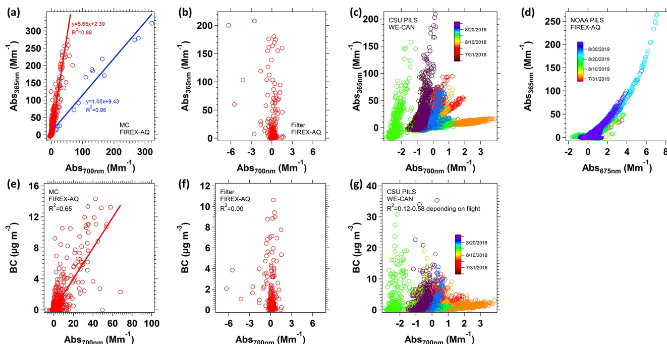
Figure 5. Scatter plots between \text{Abs}_{365\text{ nm}} and baseline ( \text{Abs}_{700\text{ nm}} ; \text{Abs}_{675\text{ nm}} for NOAA PILS) with (a) MC, (b) filter, (c) CSU PILS and (d) NOAA PILS. The corresponding scatter plots between \text{Abs}_{700\text{ nm}} and BC are shown in (e)–(g). For the (a) MC-LWCC system, two groups of data are classified visually and fit with an orthogonal distance regression. Red data are the baseline drift due to BC passing the particle filter, and blue data are because of small air bubbles in the LWCC. For PILS-LWCC (c, d), data are color-coded by sampling date.
