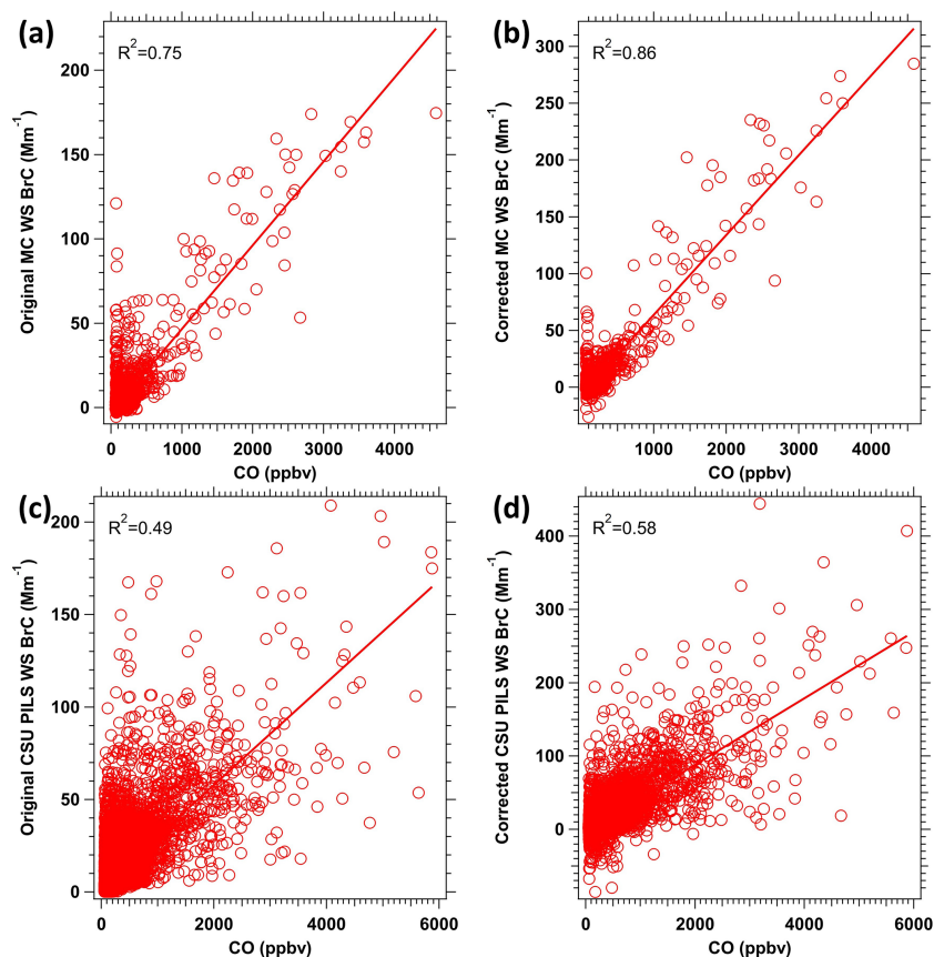
Figure 7. Scatter plots of WS BrC versus CO concentration for the MC-LWCC before (a) and after the (b) hysteresis correction and for the CSU PILS-LWCC before (c) and after the (d) hysteresis correction.
