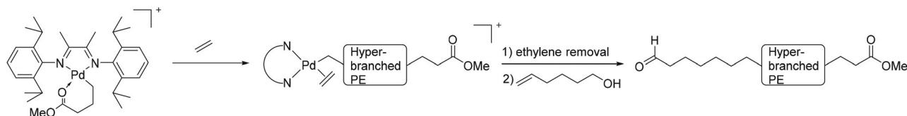
Fig. 4 Living ethylene polymerization end-capped by 5-hexenyl-1-ol. Adapted with permission from ref. 49. Copyright ACS 2020.
