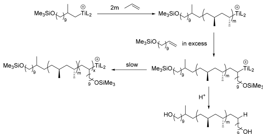
Fig. 5 Syndiotactic hydroxy-telechelic PP synthesized from functionalized initiators and end-capping reagents. Adapted with permission from ref. 50. Copyright Wiley VCH 2007.
