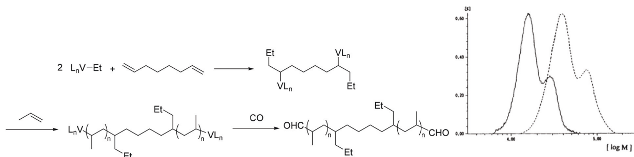
Fig. 7 Reaction scheme of propylene polymerization with binuclear vanadium complex (left) and molecular weight distribution (right). Solid line: propylene polymerization at -78\text{ }^{\circ}\text{C} . Dashed line: propylene polymerization at -65\text{ }^{\circ}\text{C} followed by CO quenching. Adapted with permission from ref. 54. Copyright Wiley VCH 1998.
