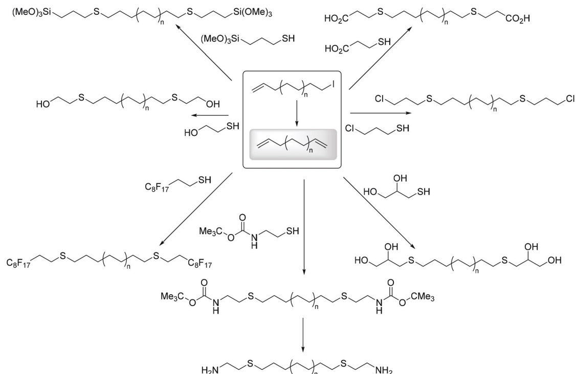
Fig. 9 Telechelic PE obtained from thiol-ene reaction of various functional thiols with divinyl telechelic PE. Adapted with permission from ref. 61. Copyright Wiley VCH 2015.
