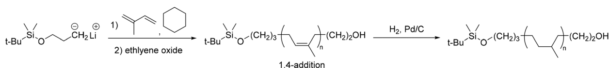
Fig. 3 Using functionalized initiator and end-capping to access hetero-telechelic poly(ethylene- alt -propylene). Adapted with permission from ref. 41. Copyright ACS 2006.
