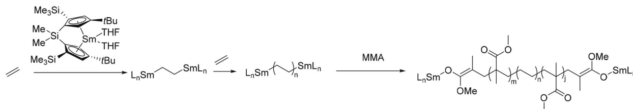
Fig. 6 PE-containing triblock copolymer from binuclear samarocene-initiated polymerization. Adapted with permission from ref. 52. Copyright Wiley VCH 2000.
