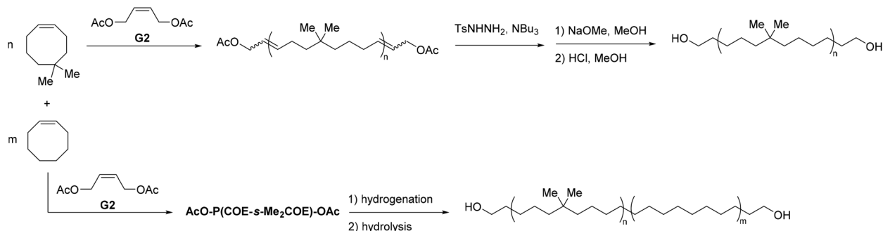
Fig. 2 Hydroxy-telechelic poly(ethylene-co-isobutylene) through ROMP. Adapted with permission from ref. 22. Copyright RSC 2015.
