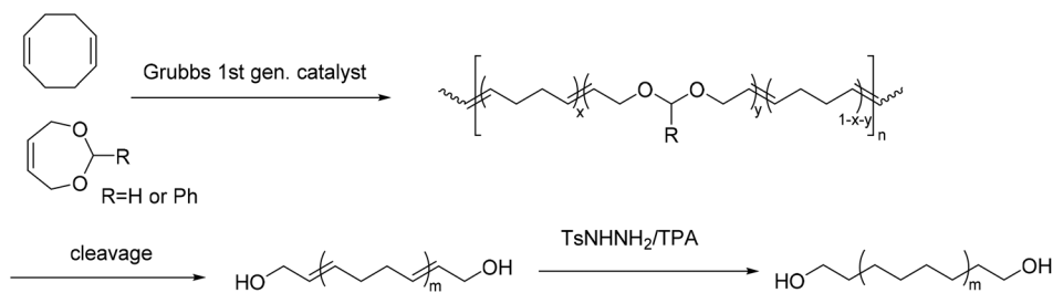
Fig. 10 Hydroxy-telechelic PE synthesized from ROMP with cyclic acetal comonomer. Adapted with permission from ref. 81. Copyright ACS 1995.
