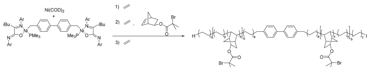
Fig. 8 Living sequential polymerization starting from binuclear nickel complex. Adapted with permission from ref. 55. Copyright ACS 2010.
