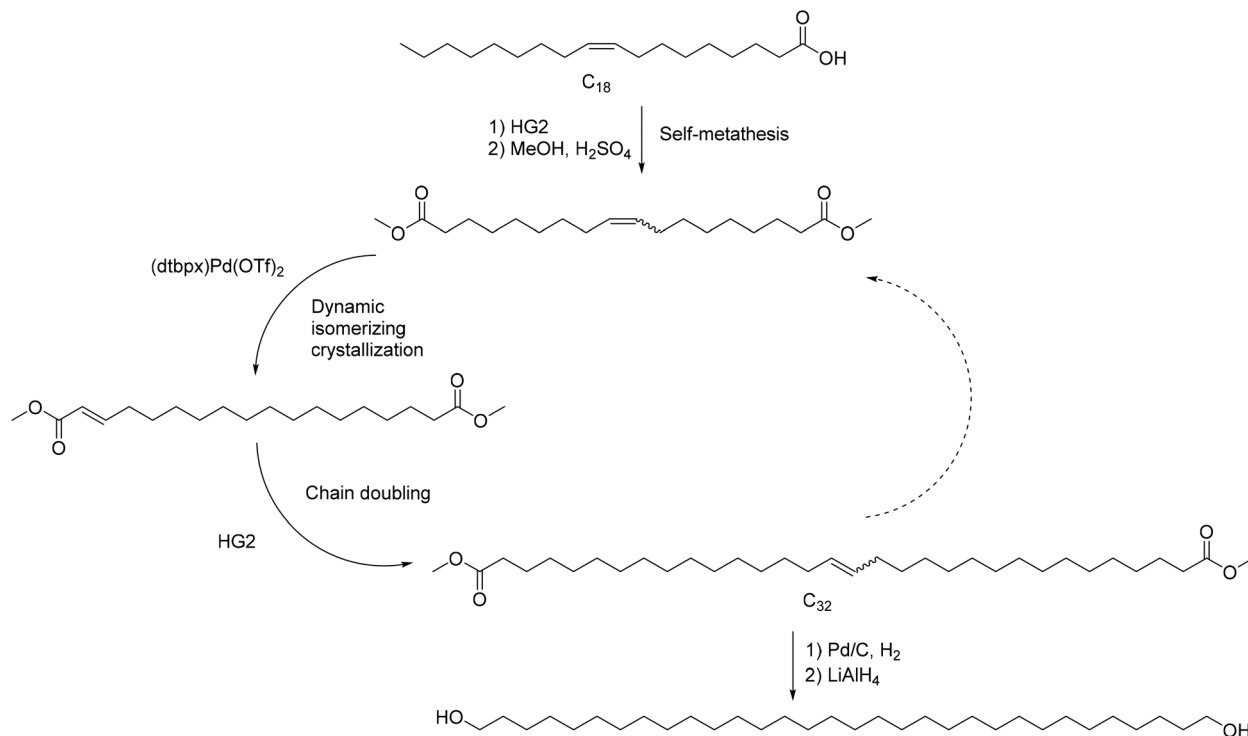
Fig. 12 The “Chain multiplication” strategy for the preparation of ultra-long-chain diester and diol. Adapted with permission from ref. 86. Copyright Wiley VCH 2017.
