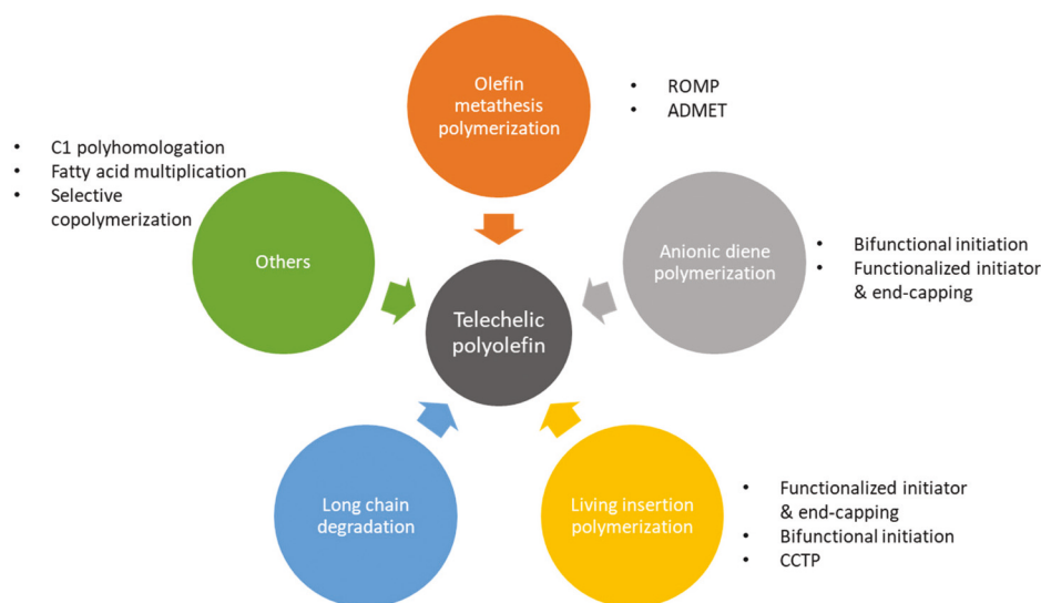
Fig. 1 Synthetic strategies for telechelic polyolefins.
