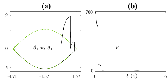
Fig. 3 Plots showing (a) phase portrait of passive joint angle \theta_1 , and (b) variation of the Lyapunov-like function V . The desired level set is shown using dashed green line in (a)
