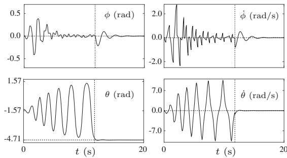
Fig. 6 Rotary pendulum simulation results
