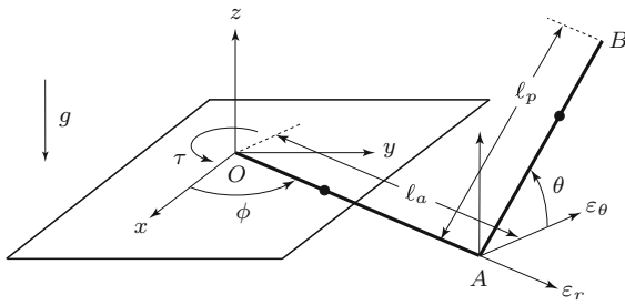
Fig. 4 Schematic of a rotary pendulum
