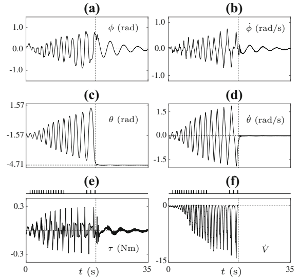
Fig. 5 Rotary pendulum experimental results: (a–d) are plots of joint angles and joint velocities, (e) control torque, and (f) derivative of Lyapunov-like function. The brake pulses are shown within plots e and f, the peaks represent time intervals when the brakes were engaged
