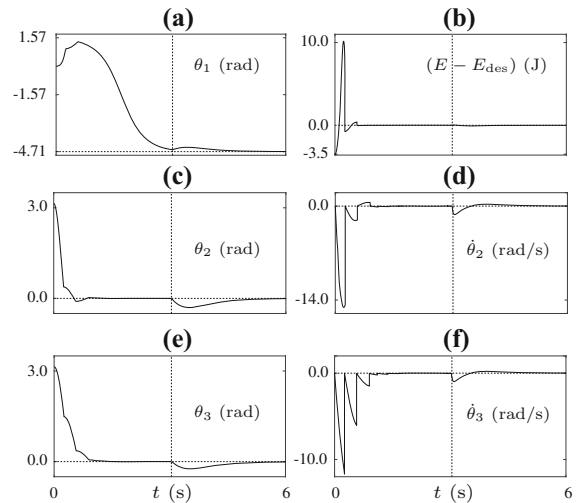
Fig. 2 Plots of the joint angles \theta_1 , \theta_2 , \theta_3 , error in the desired energy (E - E_{\text{des}}) , and the active joint velocities \dot{\theta}_2 , \dot{\theta}_3 of the Tiptoebot
