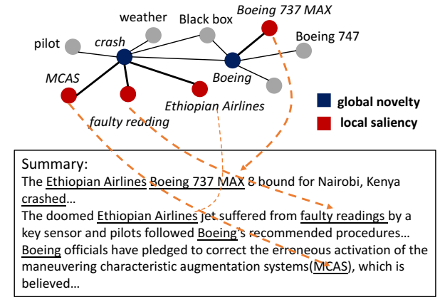
Figure 2: Text co-occurrence graph of the target documents. Global novelty are binary labels obtained from sibling documents. The scores are calculated as the difference between target and twin documents.
