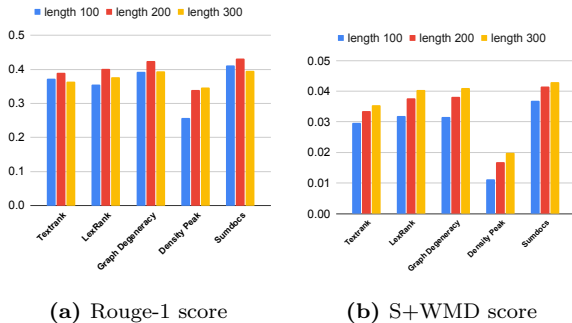
Figure 4: Performance of different methods on Scientific-NLP dataset varying length of output summary.
