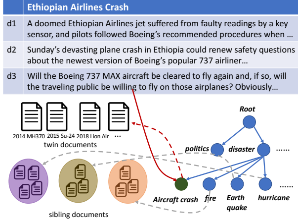
Figure 1: Examples of Surrounding Documents
