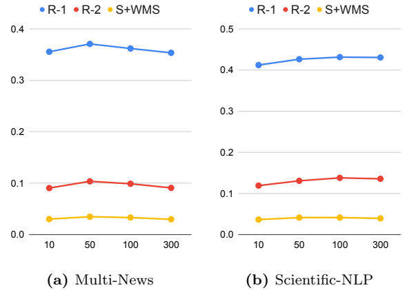
Figure 3: Performance of SUMDocS varying number of keywords used in submodular selection.
