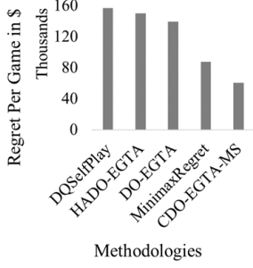
Figure 4. Regret Comparison Figure 5. CDO-EGTA Regret by No. of Clusters
