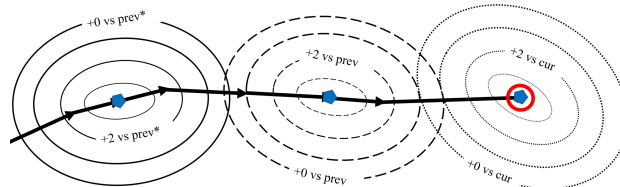
Figure 2. Conceptual Diagram of DO-EGTA
