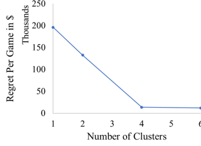
Figure 4. Regret Comparison Figure 5. CDO-EGTA Regret by No. of Clusters
