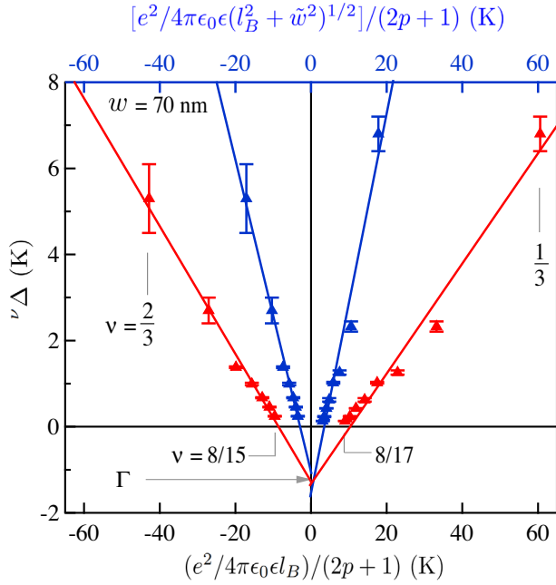
FIG. 4. Red symbols are \nu\Delta versus (e^2/4\pi\epsilon_0\epsilon l_B)/(2p + 1) , for a 2DES with w = 70 nm. The \nu range is from 1/3 to 8/17 , and 2/3 to 8/15 . The red lines are linear fits to the data. The blue symbols are \nu\Delta versus the Zhang–Das Sarma energy [e^2/4\pi\epsilon_0\epsilon(l_B^2 + \tilde{w}^2)^{1/2}]/(2p + 1) . The blue lines are linear fits to the blue data points. The red and blue lines have negative intercept values with the y axis that we identify as the phenomenological disorder parameter ( \Gamma ).
