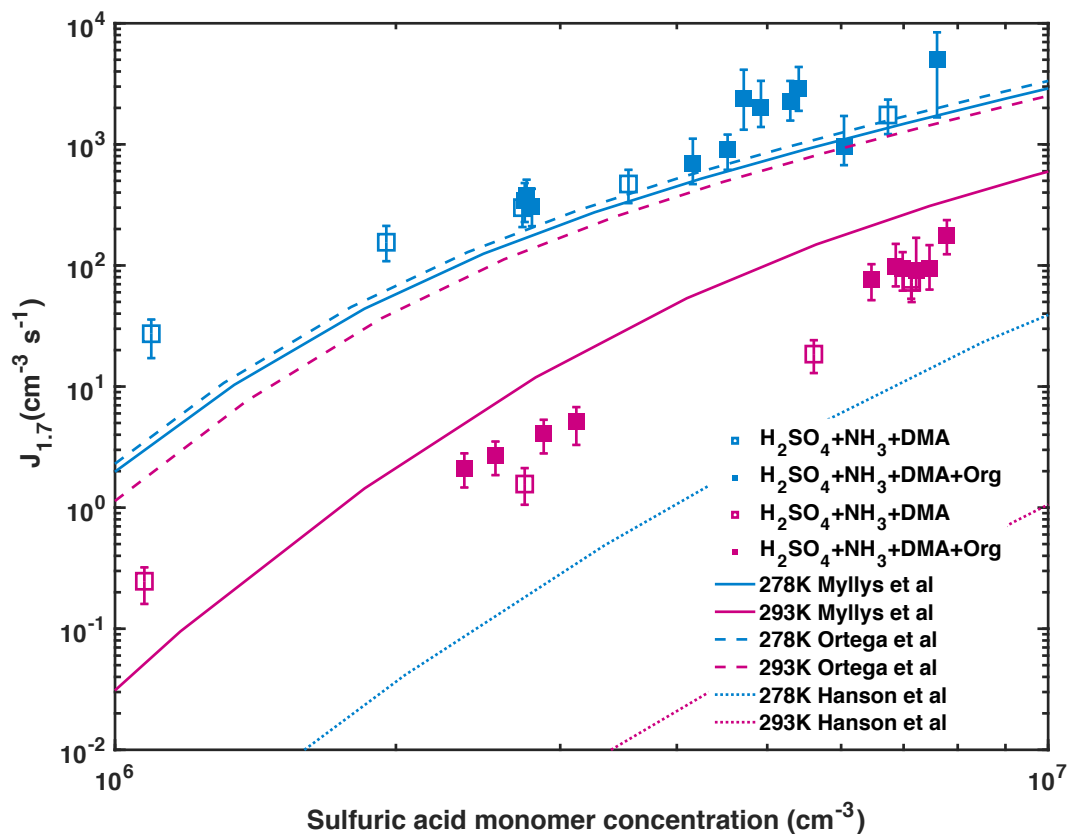
Figure S1: Modelled particle formation rates at 1.7 nm diameter from sulfuric acid with \text{NH}_3 and DMA compared with our measurements at 293 and 278 K. Experiments were performed at 278 K (cyan) or 293 K (magenta) with 1 to 2 ppbv \text{NH}_3 and 4 pptv DMA. Filled and open symbols indicate presence or absence of organics, respectively. The error bars refer to the measurement uncertainties for the particle formation rates. Solid and dashed lines are calculated with the kinetic model by implementing sulfuric acid - DMA cluster evaporation rates based on thermodynamic data from Myllys et al. (2019) (solid line), Ortega et al. (2012) (dashed line) and from Hanson et al. (2017) (dotted line), respectively. Modelled results based on binding energies for \text{H}_2\text{SO}_4 -DMA clusters from Myllys et al (2019). follow the same trends as our measurements while other published binding energies for \text{H}_2\text{SO}_4 -DMA clusters fail to reproduce the temperature dependency of the measured J_{1.7} . The tightly bound clusters theoretically predicted by Ortega et al. (2012) result in minor evaporation, leading to formation rates close to kinetic limits even at high temperatures. Note that the quantum chemical method used tends to overestimate binding energy values (Leverentz et al., 2013), and a reduction of the values at 298 K for the \text{H}_2\text{SO}_4 -DMA cluster (-15.4 to -11 \text{kcal mol}^{-1} ) and for (\text{H}_2\text{SO}_4)_2 -DMA (-19.48 to -18 \text{kcal mol}^{-1} ), as suggested by Hanson et al. (2017), results in considerably lower J_{1.7} values compared to our observations.
