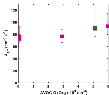
50 Figure S3. Dependence of particle formation rates from sulfuric acid, ammonia, DMA, and AVOC on OxOrg concentration at (A) 293 K and (B) 278 K. (A) Experiments with 7.4 \pm 0.4 \times 10^6 \text{ cm}^{-3} \text{ H}_2\text{SO}_4 , 800 to 2000 pptv \text{NH}_3 , 4 pptv DMA and 0.71 \pm 0.18 \text{ ppbv NO} at 293 K, with NAPH:TMB:TOL of 1:5:15. Symbol highlighted with green outline also has 1 ppbv \alpha -pinene added to the experiment. Error bars present variation of the measurements. (B) Experiments with 5.1 \pm 0.6 \times 10^6 \text{ cm}^{-3} \text{ H}_2\text{SO}_4 , 1000 to 1500 pptv \text{NH}_3 , 4 pptv DMA and 0.67 \pm 0.4 \text{ ppbv NO} at 293 K, with NAPH:TMB:TOL of 1:5:20. Symbol highlighted with green outline also has 1 ppbv \alpha -pinene added to the experiment. Error bars present variation of the measurements. 55
