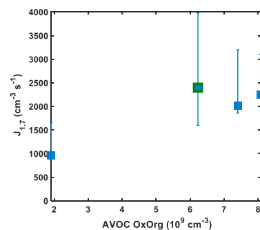
50 Figure S3. Dependence of particle formation rates from sulfuric acid, ammonia, DMA, and AVOC on OxOrg concentration at (A) 293 K and (B) 278 K. (A) Experiments with 7.4 \pm 0.4 \times 10^6 \text{ cm}^{-3} \text{ H}_2\text{SO}_4 , 800 to 2000 pptv \text{NH}_3 , 4 pptv DMA and 0.71 \pm 0.18 \text{ ppbv NO} at 293 K, with NAPH:TMB:TOL of 1:5:15. Symbol highlighted with green outline also has 1 ppbv \alpha -pinene added to the experiment. Error bars present variation of the measurements. (B) Experiments with 5.1 \pm 0.6 \times 10^6 \text{ cm}^{-3} \text{ H}_2\text{SO}_4 , 1000 to 1500 pptv \text{NH}_3 , 4 pptv DMA and 0.67 \pm 0.4 \text{ ppbv NO} at 293 K, with NAPH:TMB:TOL of 1:5:20. Symbol highlighted with green outline also has 1 ppbv \alpha -pinene added to the experiment. Error bars present variation of the measurements. 55
