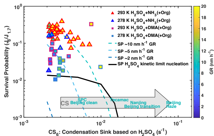
Figure S4. Enhanced growth rates of sub-3 nm particles by OxOrg. CLOUD data recorded at 278 K (blue and cyan) or 293 K (red and magenta) with 1 \times 10^6 to 1 \times 10^8 \text{cm}^{-3} \text{H}_2\text{SO}_4 and 1 to 2 ppbv \text{NH}_3 at GCR conditions. Experiments without DMA are shown by triangles, and with 4 pptv DMA by squares. Enhanced growth rates are calculated as measured growth rates minus the growth rates resulting from condensing sulfuric acid alone. Solid lines display the percentage contribution of 0.5, 1, and 3% of OxOrg to the growth rate. No \text{NO}_x dependence can be identified. The variability in condensable OxOrg yields is driven by \text{NO}_x concentrations, multi-generation chemistry and precursor composition, e.g., naphthalene oxidation leads to lower volatility products than the single-ring aromatics.
