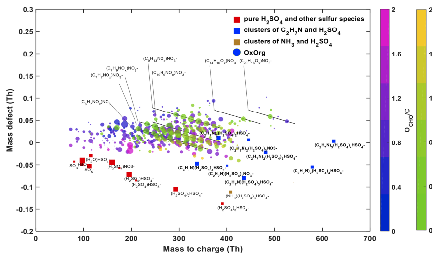
Figure 6. Mass defect plot of sulfuric acid nucleation with DMA in the presence of organics at 278 K in the CLOUD chamber. The conditions are 5.2 \times 10^6\ cm^{-3} H_2SO_4 monomer, 4 pptv DMA, 1200 pptv NH_3 , 680 pptv NO, 420 pptv NAPH, 2200 pptv TMB and 9250 pptv TOL. Sulfate clusters are shown by red squares, sulfate–DMA clusters containing up to 5 sulfur molecules by blue squares, sulfate– NH_3 clusters by brown squares, and organics by circles coloured by O : C and by their chemical composition CHO or CHNO, respectively. The size of the symbols is proportional to their intensity in the mass spectrum.
