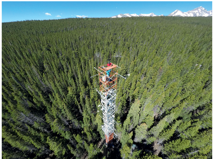
Fig. 1. Troy Magney and Katja Grossmann maintain an SIF-enabled spectrometer on a tall tower used to measure \text{CO}_2 at Niwot Ridge, Colorado. Surface trace-gas exchange measurements using a combination of techniques allow us to compare traditional to cutting-edge datasets and benchmark new observations from satellites. Photo courtesy of Christian Frankenberg.
