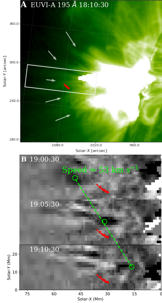
Figure 11. Example of plasma downflows observed in STEREO-A/EUVI 195 Å images. (a) Spike burst location at 18:07:07 UT (same as those in Fig. 9(b)) overlaid on EUVI 195 Å. The diffuse SAF structure is indicated by white arrows. (b) Example plasma downflow observed in the vicinity of the spike burst at 19:00–19:10 UT. The field of view is indicated by a white box in panel (a). To show the downflow feature more clearly, running-ratio images are used. Note that although the downflows are tracked using dark moving features (green circle) in the running-ratio images, similar to those in AIA 131 Å, they are in fact bright moving features in the original images. The speed in projection of this downflow is \sim 53 \text{ km s}^{-1} . An animation of the example downflow from 18:35:30 UT to 19:20:30 UT is available online. The duration of the animation is 2 s.
