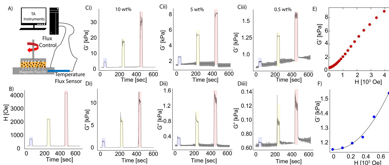
Figure 1. Magnetorheological characterization of common hydrogels and model validation. (A) Magnetorheology test setup with axial application of the magnetic field to hydrogels within a cone and plate geometry. (B) Variation of the magnetic field controlled by the magnetorheometer. Collagen hydrogel storage moduli with (Ci) 10, (Cii) 5, and (Ciii) 0.5 wt % MPs. Loss moduli of (Di) 10, (Dii) 5, and (Diii) 0.5 wt % MPs. Data presented as mean \pm s.d. ( n = 3 ). (E) Dependence of 1 mg/mL fibrin storage modulus on magnetic field strength. (F) Measurement of the PDMS storage modulus, embedded with 10 wt % MPs, as a function of the magnetic field (blue circles) and prediction of the analytical model (line).
