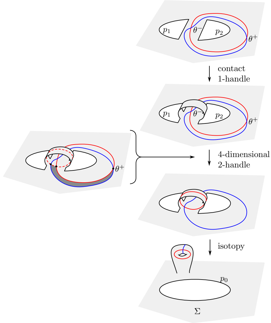
Figure 4.4. Computing the merge map. On the left side, an index 0 holomorphic triangle is shown.
