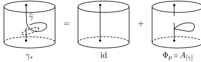
Figure 6.2. Obtaining the formula for the \pi_1 -action by applying the local relation from Figure 6.1 to the graph \hat{\gamma} .
