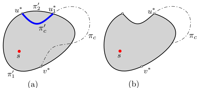
Figure 4: (a) The cycle \gamma with |\gamma \cap \pi_c| = 4 . Here, \gamma_1 = \pi'_1 \oplus \pi'_c is also a separating cycle. (b) The cycle \gamma_1 with |\gamma_1 \cap \pi_c| = 3 . The shortcut-path \pi_c is shown dash-dotted.
