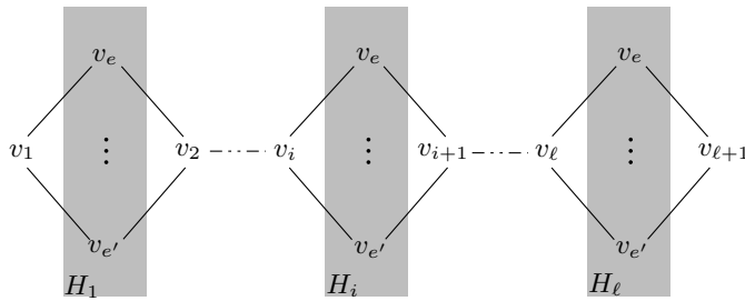
Figure 6: An example of the construction. The groups H_1, H_i and H_\ell are shown shaded in gray.
