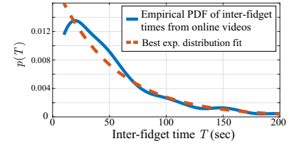
Figure 11: The exponential distribution well fits the empirical PDF of the collected individual inter-fidget times of 6 subjects, showing that the Poisson process well describes the individual fidgeting process.
