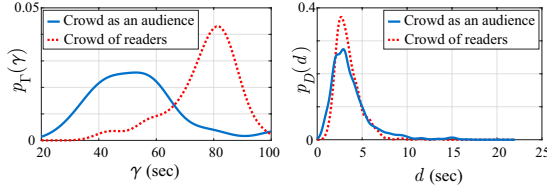
Figure 5: (Left) The distribution of the average inter-fidget time of an individual, p_T(\gamma) , for a general population, collected from the data of a total of 30 individuals attending various events in 14 public online Youtube videos (for the case of audience), and 24 individuals reading in 24 different online YouTube videos (for the case of readers). It can be seen that people tend to fidget less when reading, since it requires more focus. (Right) The distribution of the fidget duration p_D(d) of an individual, estimated from the same dataset.
