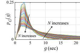
Figure 6: PDF of the duration of a CFP of the aggregate process ( p_G(g) ), from Eq. 3, as a function of N and for an audience-style activity. The figure explicitly shows the dependence of the duration of a CFP on the number of people, which is characterized through our proposed mathematical framework. Higher N results in a higher probability of having longer CFPs, as can be seen.
