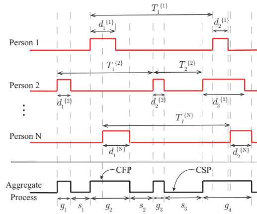
Figure 2: A sample fidgeting timeline of N people in an area, where a non-zero signal indicates a fidget. d_i^{(n)} denotes the duration of the i -th fidget of the n -th person, while T_i^{(n)} represents the time between the i -th and (i + 1) -th fidgets of the n -th person. An aggregate fidgeting process results from the superposition of the individual fidgeting processes, where the state of no one fidgeting is referred to as the Crowd Silent Period (CSP) (with a duration s ), while the state of at least one person fidgeting is referred to as the Crowd Fidgeting Period (CFP) (with a duration g ). A sample CFP and CSP are marked on the figure.
