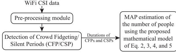
Figure 3: High-level overview of the proposed pipeline.
